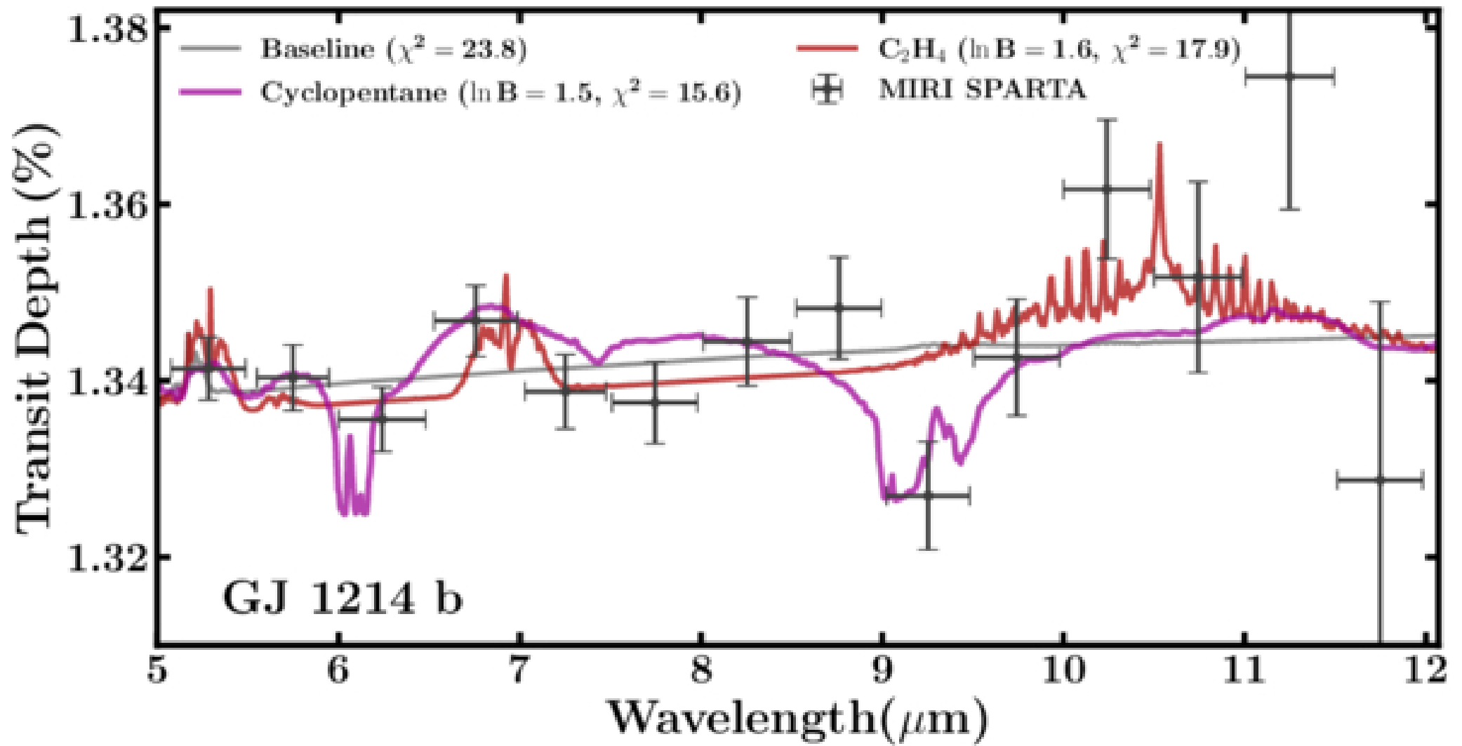
Figure 11. from Martin Binet et al 2026 Astrophys. J. Lett. 1008 doi:10.3847/2041-8213/ae8c2d https://dx.doi.org/10.3847/2041-8213/ae8c2d © 2026. The Author(s). Published by the American Astronomical Society.
