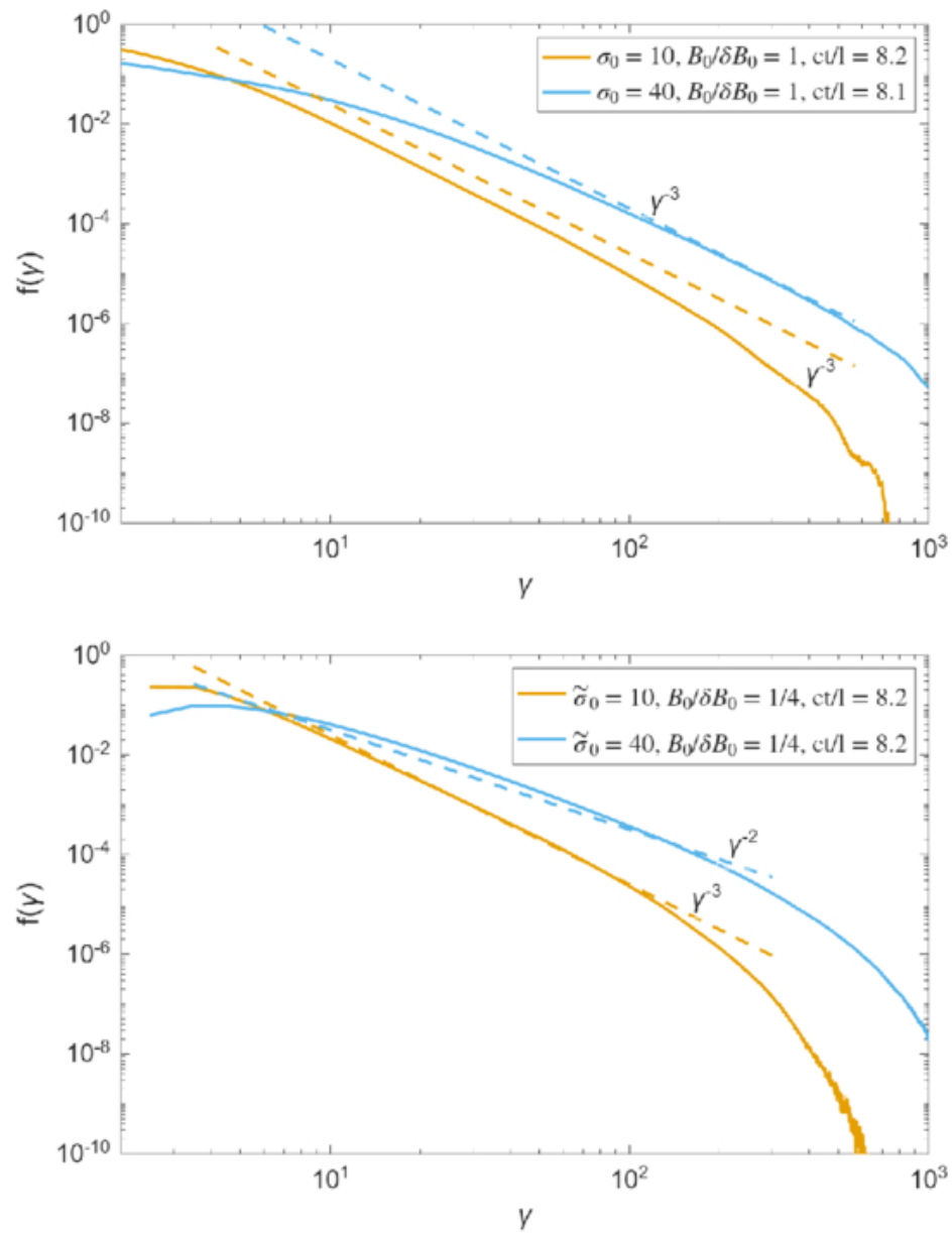
Figure 1. from Stanislav Boldyrev et al 2026 Astrophys. J. Lett. 1007 doi:10.3847/2041-8213/ae8bac https://dx.doi.org/10.3847/2041-8213/ae8bac © 2026. The Author(s). Published by the American Astronomical Society.
