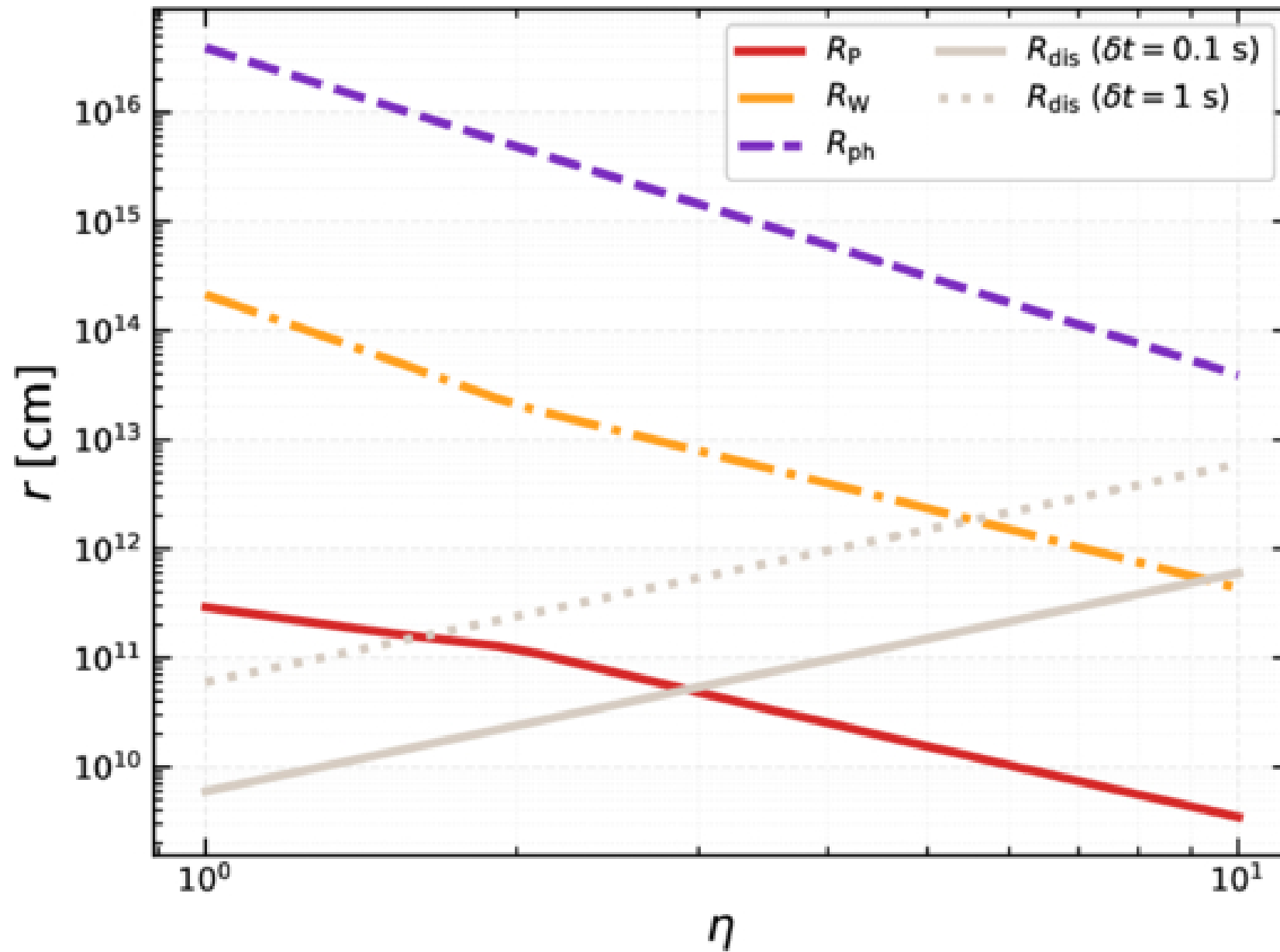
Figure 5. from Cui-Yuan Dai et al 2026 Astrophys. J. Lett. 1006 doi:10.3847/2041-8213/ae8ba8 https://dx.doi.org/10.3847/2041-8213/ae8ba8 © 2026. The Author(s). Published by the American Astronomical Society.
