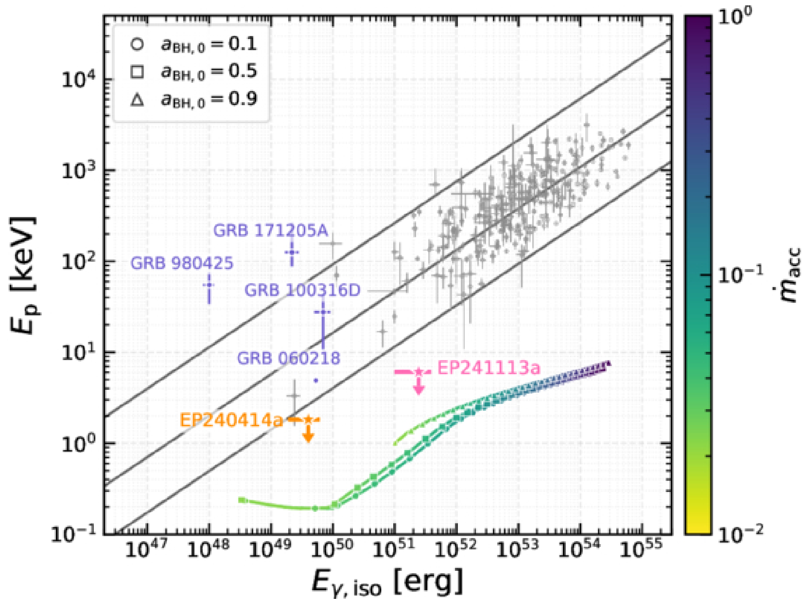
Figure 4. from Cui-Yuan Dai et al 2026 Astrophys. J. Lett. 1006 doi:10.3847/2041-8213/ae8ba8 https://dx.doi.org/10.3847/2041-8213/ae8ba8 © 2026. The Author(s). Published by the American Astronomical Society.
