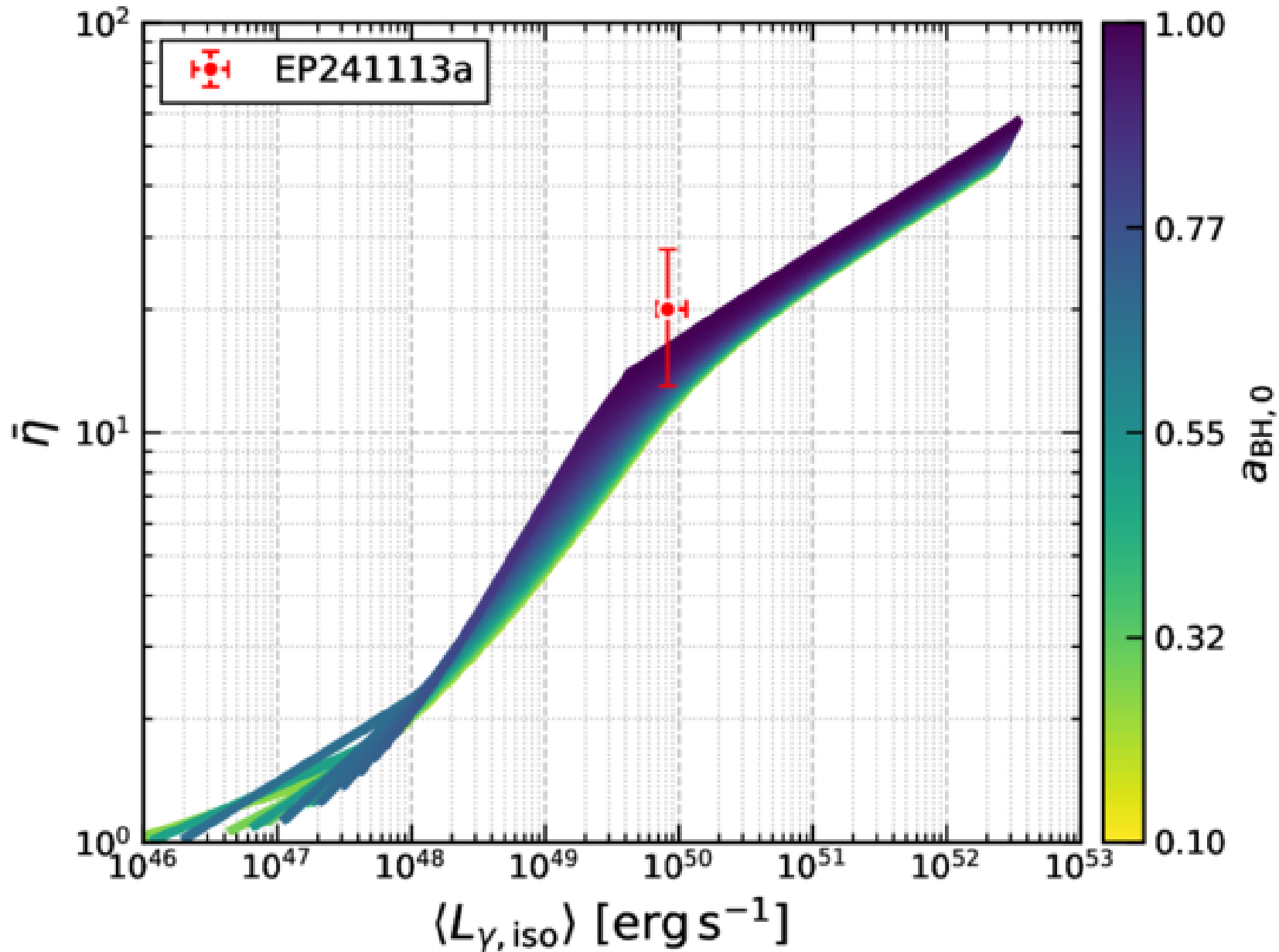
Figure 3. from Cui-Yuan Dai et al 2026 Astrophys. J. Lett. 1006 doi:10.3847/2041-8213/ae8ba8 https://dx.doi.org/10.3847/2041-8213/ae8ba8 © 2026. The Author(s). Published by the American Astronomical Society.
