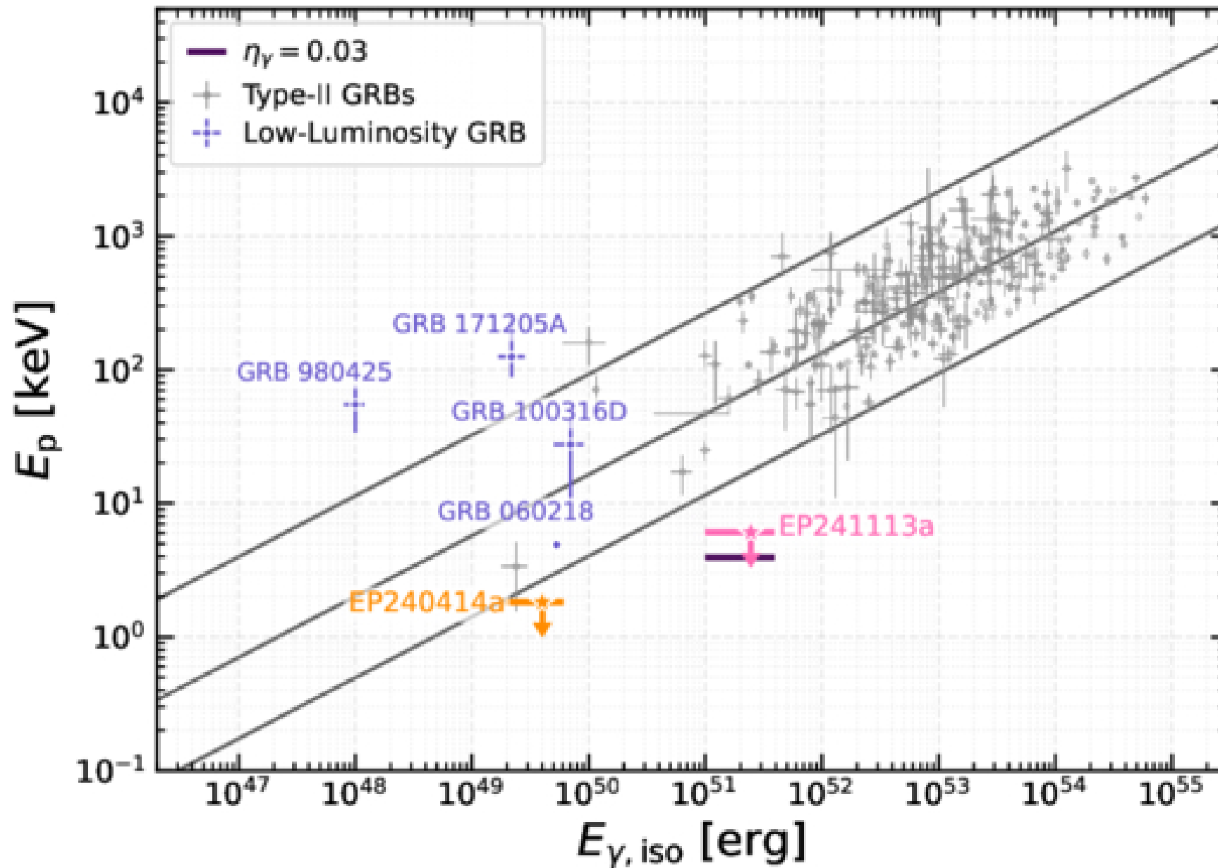
Figure 2. from Cui-Yuan Dai et al 2026 Astrophys. J. Lett. 1006 doi:10.3847/2041-8213/ae8ba8 https://dx.doi.org/10.3847/2041-8213/ae8ba8 © 2026. The Author(s). Published by the American Astronomical Society.
