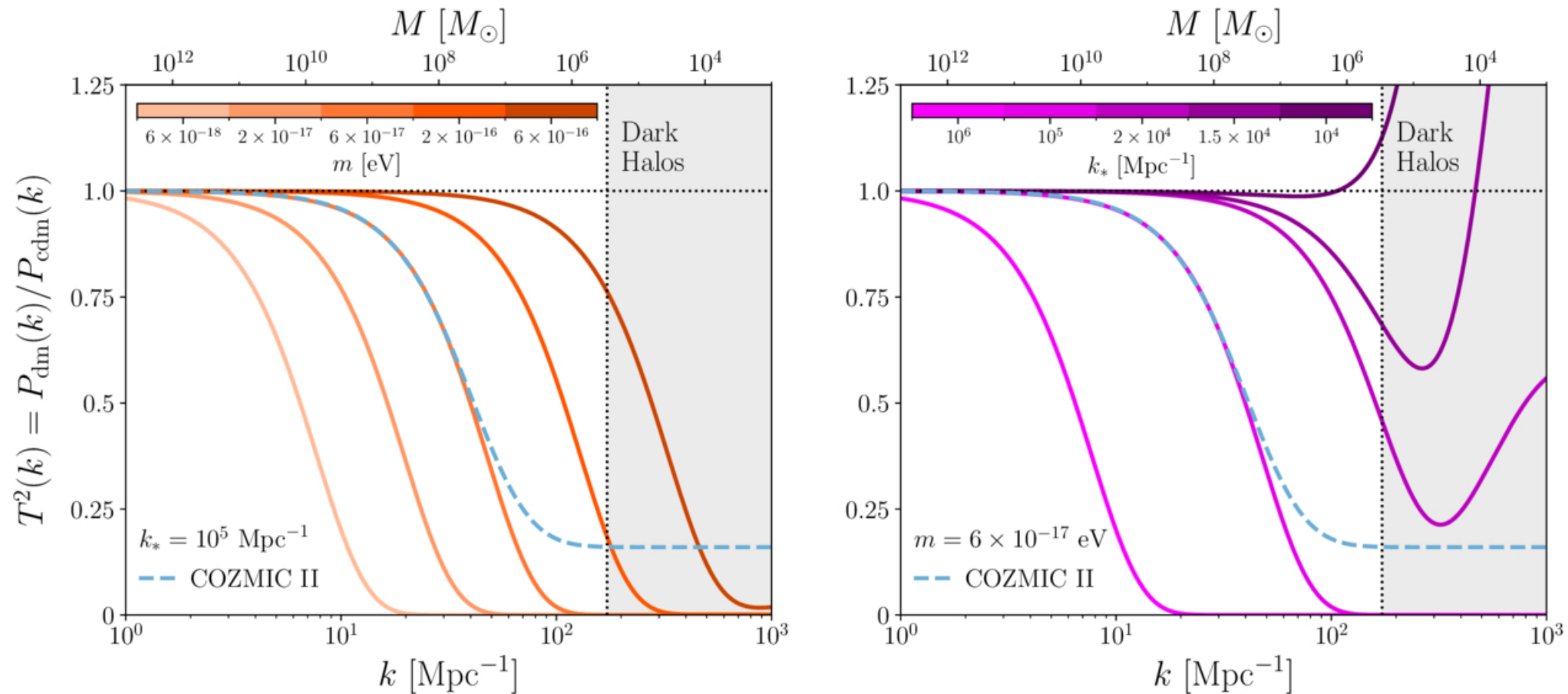
Figure 1. from Ethan O. Nadler et al 2026 Astrophys. J. Lett. 1006 doi:10.3847/2041-8213/ae8b9f https://dx.doi.org/10.3847/2041-8213/ae8b9f © 2026. The Author(s). Published by the American Astronomical Society.
