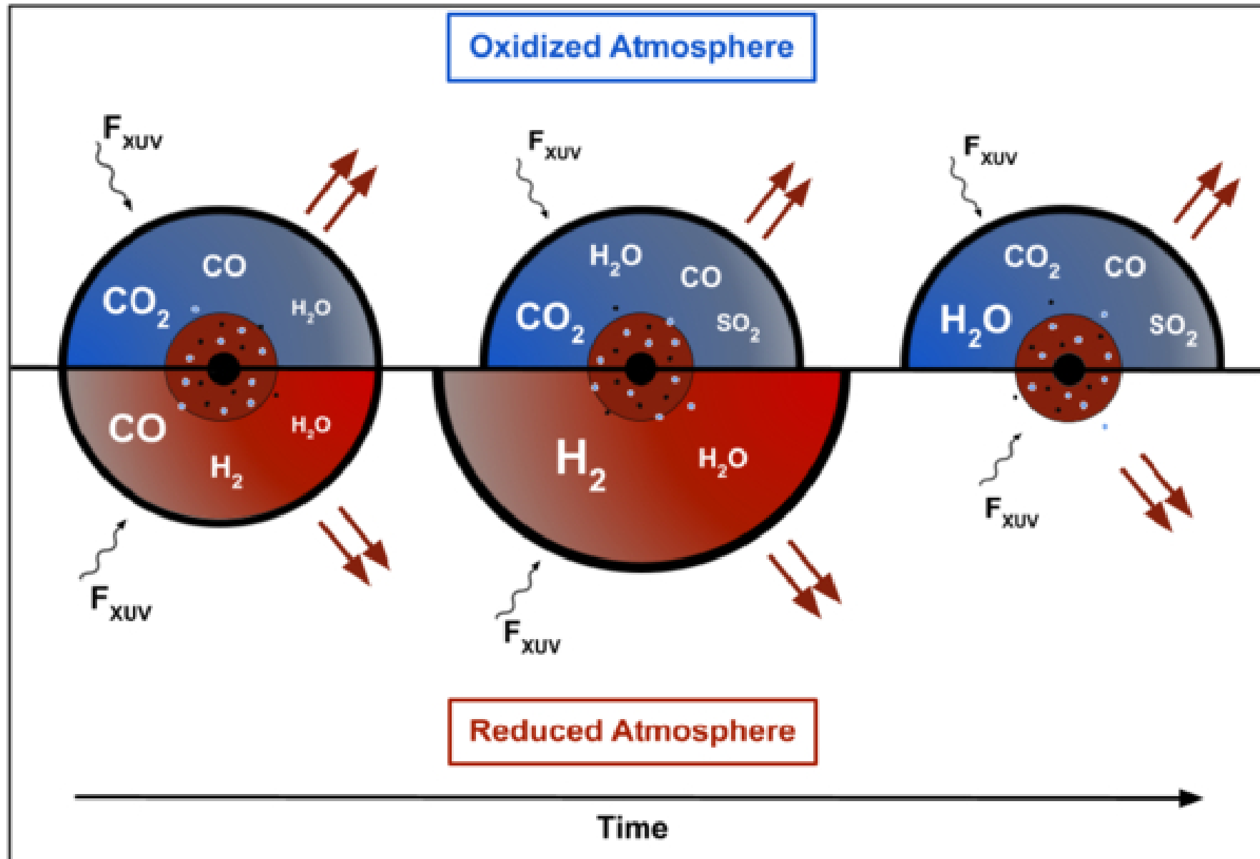
Figure 4. from Lorenzo Cesario et al 2026 Astrophys. J. Lett. 1007 doi:10.3847/2041-8213/ae8b95 https://dx.doi.org/10.3847/2041-8213/ae8b95 © 2026. The Author(s). Published by the American Astronomical Society.
