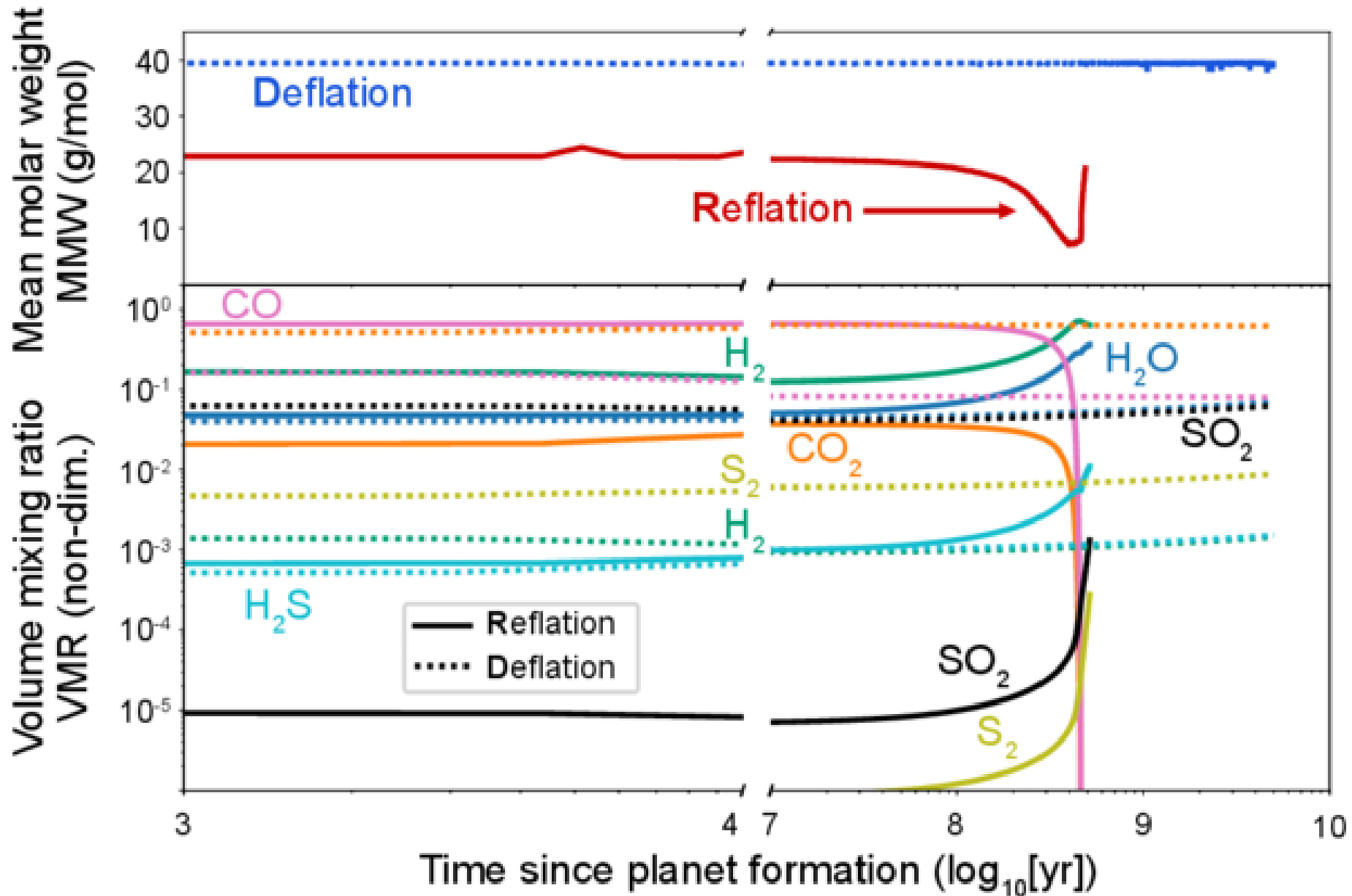
Figure 2. from Lorenzo Cesario et al 2026 Astrophys. J. Lett. 1007 doi:10.3847/2041-8213/ae8b95 https://dx.doi.org/10.3847/2041-8213/ae8b95 © 2026. The Author(s). Published by the American Astronomical Society.
