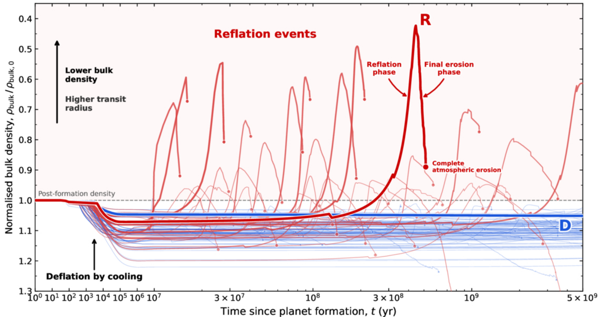
Figure 1. from Lorenzo Cesario et al 2026 Astrophys. J. Lett. 1007 doi:10.3847/2041-8213/ae8b95 https://dx.doi.org/10.3847/2041-8213/ae8b95 © 2026. The Author(s). Published by the American Astronomical Society.
