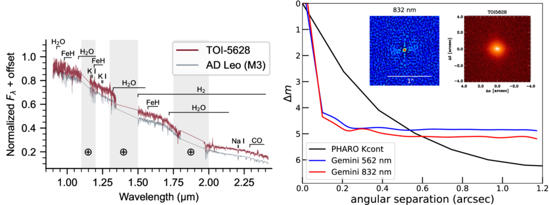
Figure A2. from Tianjun Gan et al 2026 Astrophys. J. Lett. 1006 doi:10.3847/2041-8213/ae8af1 https://dx.doi.org/10.3847/2041-8213/ae8af1 © 2026. The Author(s). Published by the American Astronomical Society.
