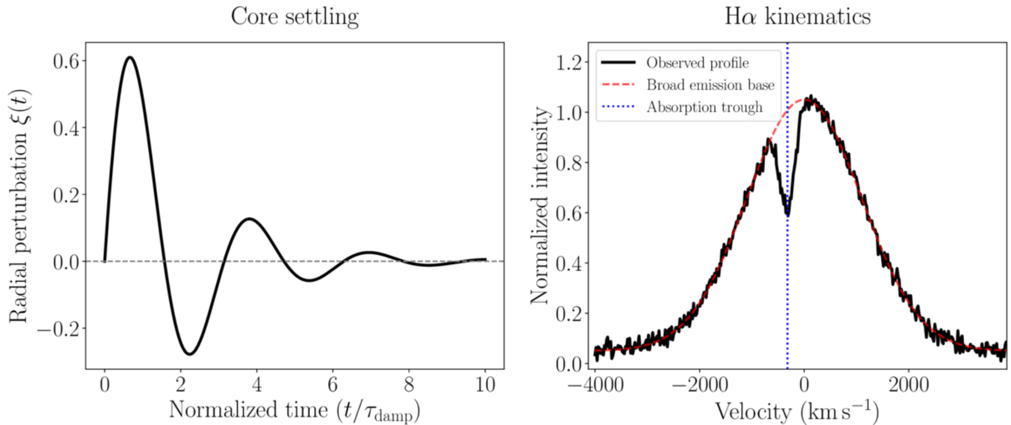
Figure 3. from Pau Amaro Seoane 2026 Astrophys. J. Lett. 1006 doi:10.3847/2041-8213/ae8aee https://dx.doi.org/10.3847/2041-8213/ae8aee © 2026. The Author(s). Published by the American Astronomical Society.
