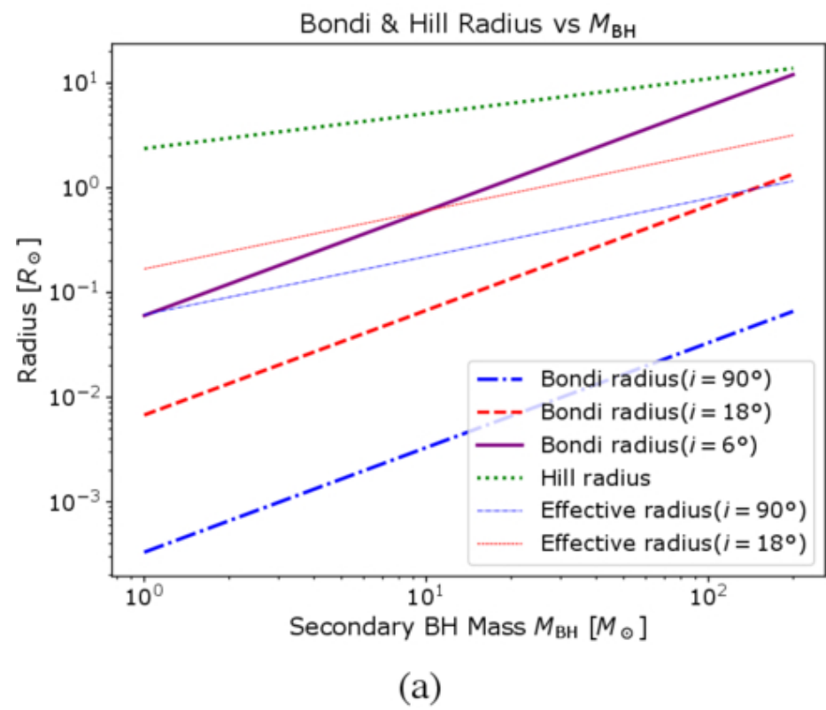
Figure 8. from Kun Liu et al 2026 Astrophys. J. Lett. 1006 doi:10.3847/2041-8213/ae8aeb https://dx.doi.org/10.3847/2041-8213/ae8aeb © 2026. The Author(s). Published by the American Astronomical Society.
