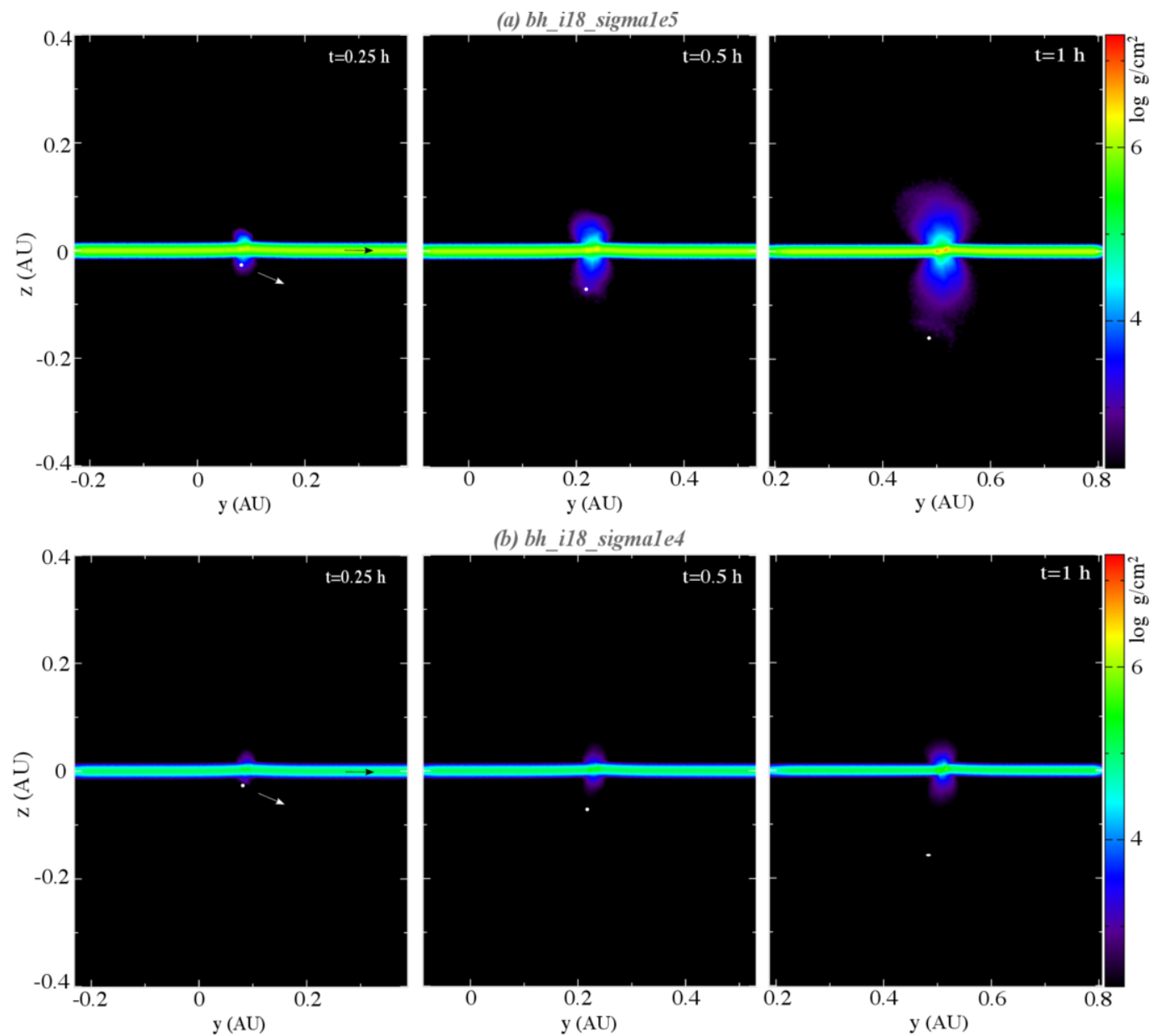
Figure 6. from Kun Liu et al 2026 Astrophys. J. Lett. 1006 doi:10.3847/2041-8213/ae8aeb https://dx.doi.org/10.3847/2041-8213/ae8aeb © 2026. The Author(s). Published by the American Astronomical Society.
