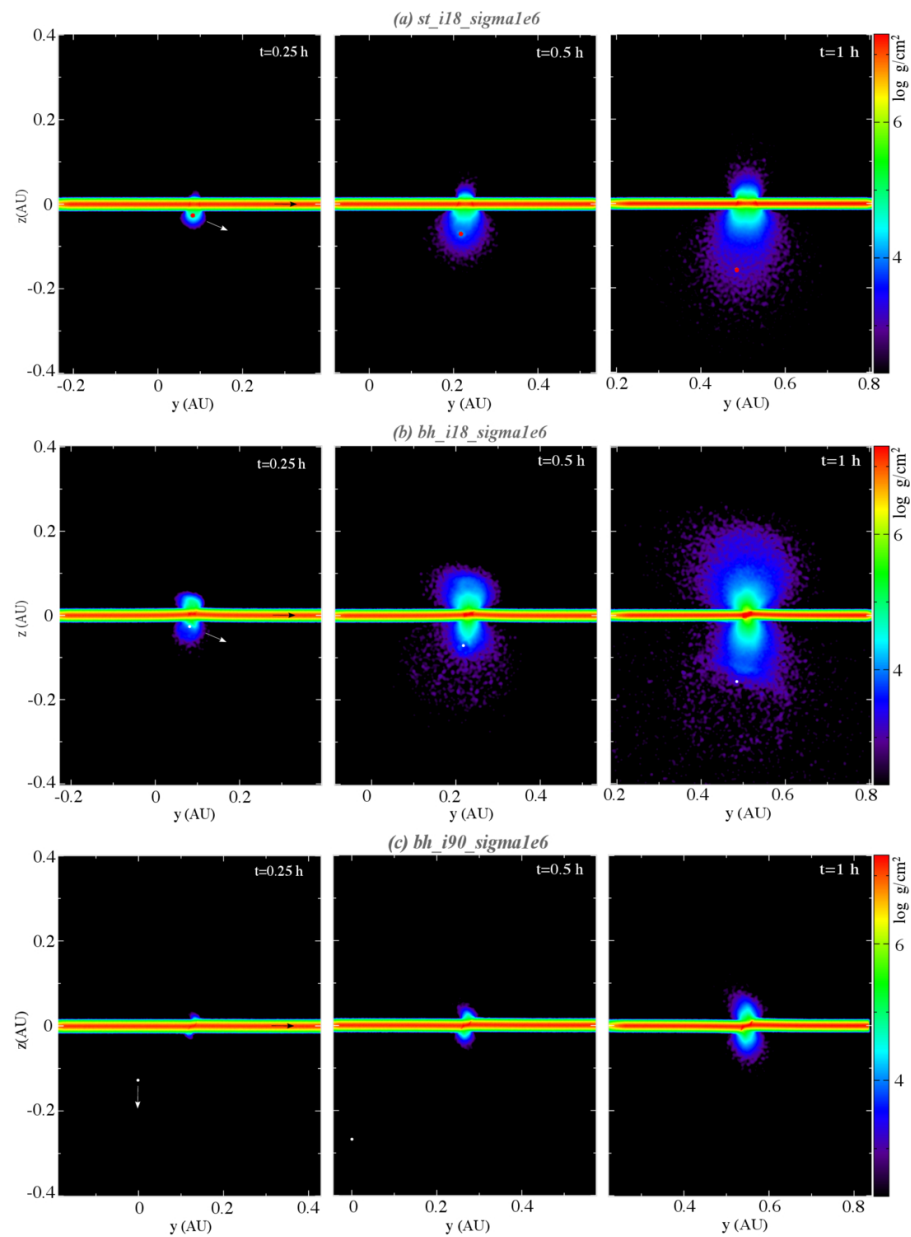
Figure 5. from Kun Liu et al 2026 Astrophys. J. Lett. 1006 doi:10.3847/2041-8213/ae8aeb https://dx.doi.org/10.3847/2041-8213/ae8aeb © 2026. The Author(s). Published by the American Astronomical Society.
