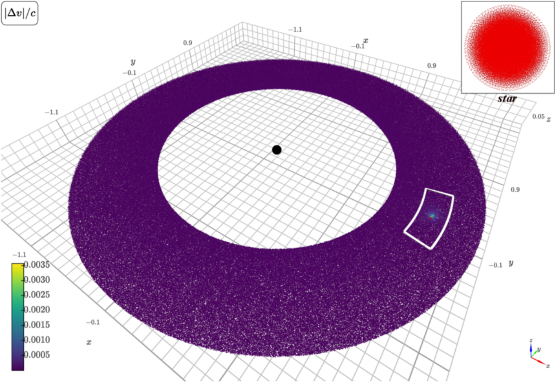
Figure 3. from Kun Liu et al 2026 Astrophys. J. Lett. 1006 doi:10.3847/2041-8213/ae8aeb https://dx.doi.org/10.3847/2041-8213/ae8aeb © 2026. The Author(s). Published by the American Astronomical Society.
