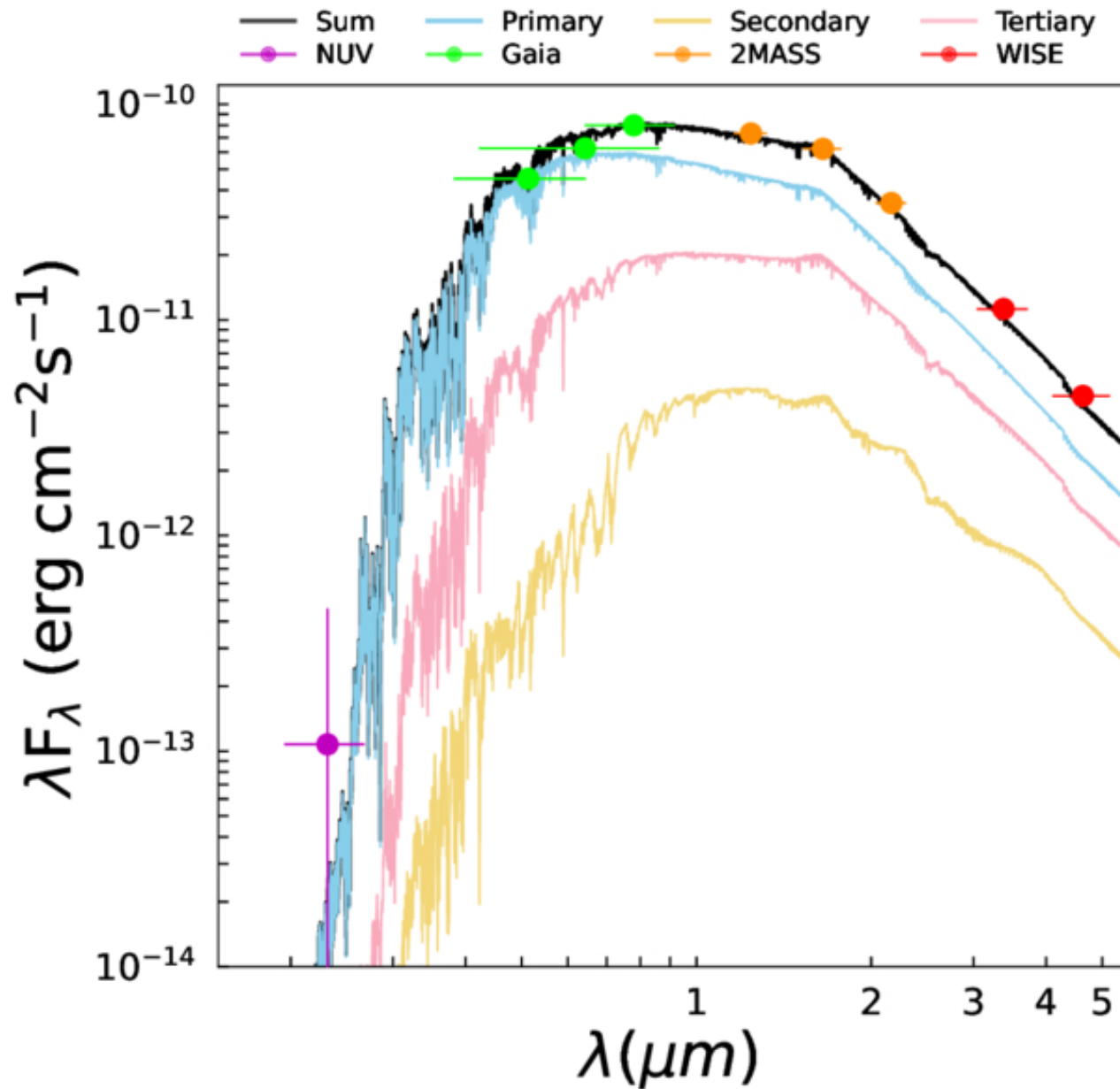
Figure 3. from Yinghao Xu et al 2026 Astrophys. J. Lett. 1006 doi:10.3847/2041-8213/ae8ae9 https://dx.doi.org/10.3847/2041-8213/ae8ae9 © 2026. The Author(s). Published by the American Astronomical Society.
