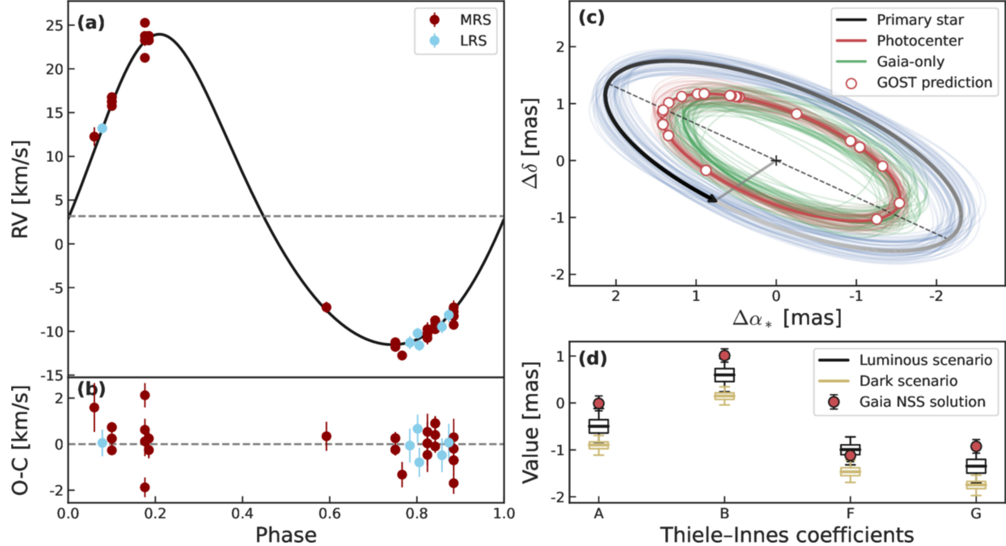
Figure 2. from Yinghao Xu et al 2026 Astrophys. J. Lett. 1006 doi:10.3847/2041-8213/ae8ae9 https://dx.doi.org/10.3847/2041-8213/ae8ae9 © 2026. The Author(s). Published by the American Astronomical Society.
