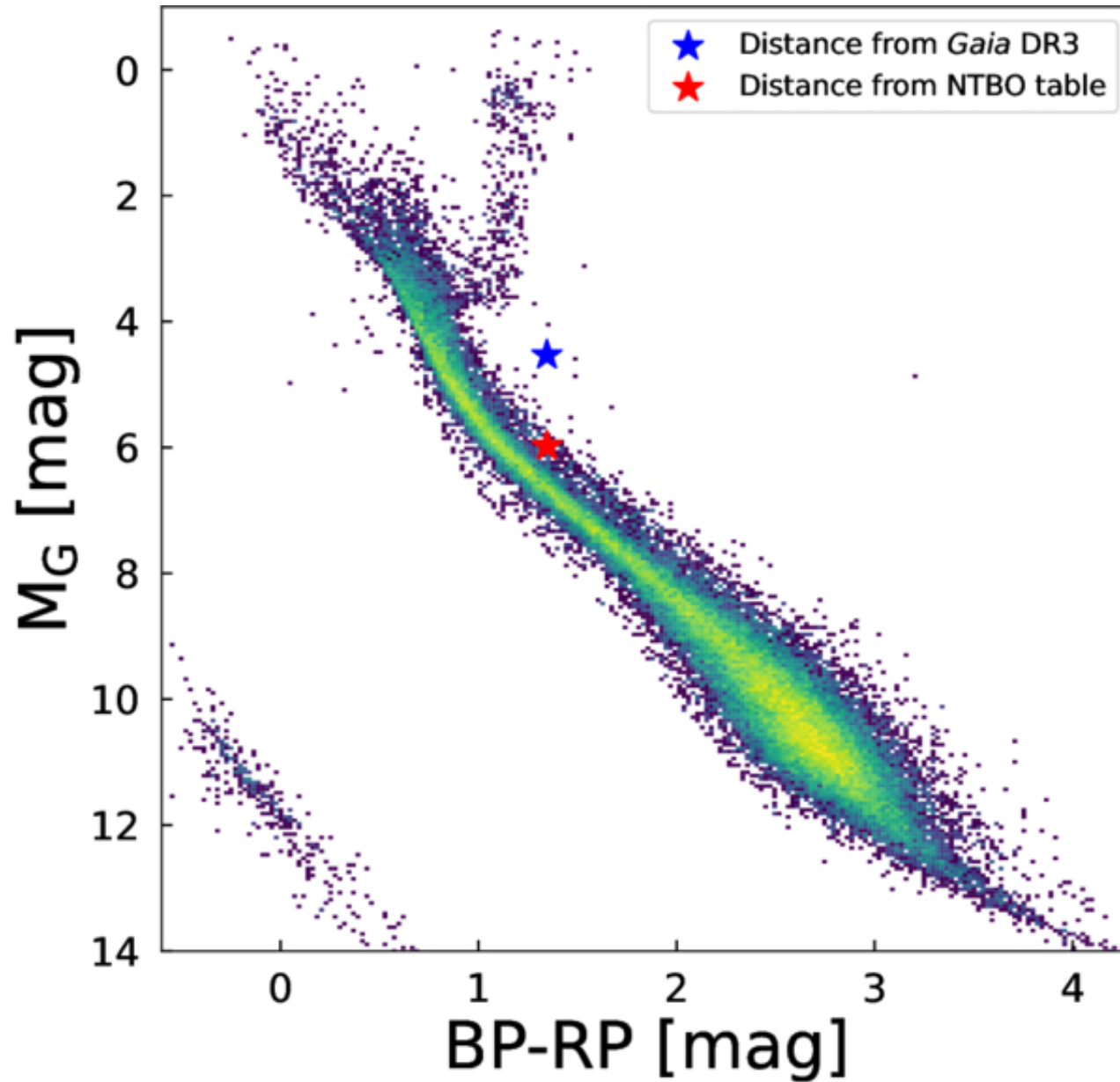
Figure 1. from Yinghao Xu et al 2026 Astrophys. J. Lett. 1006 doi:10.3847/2041-8213/ae8ae9 https://dx.doi.org/10.3847/2041-8213/ae8ae9 © 2026. The Author(s). Published by the American Astronomical Society.
