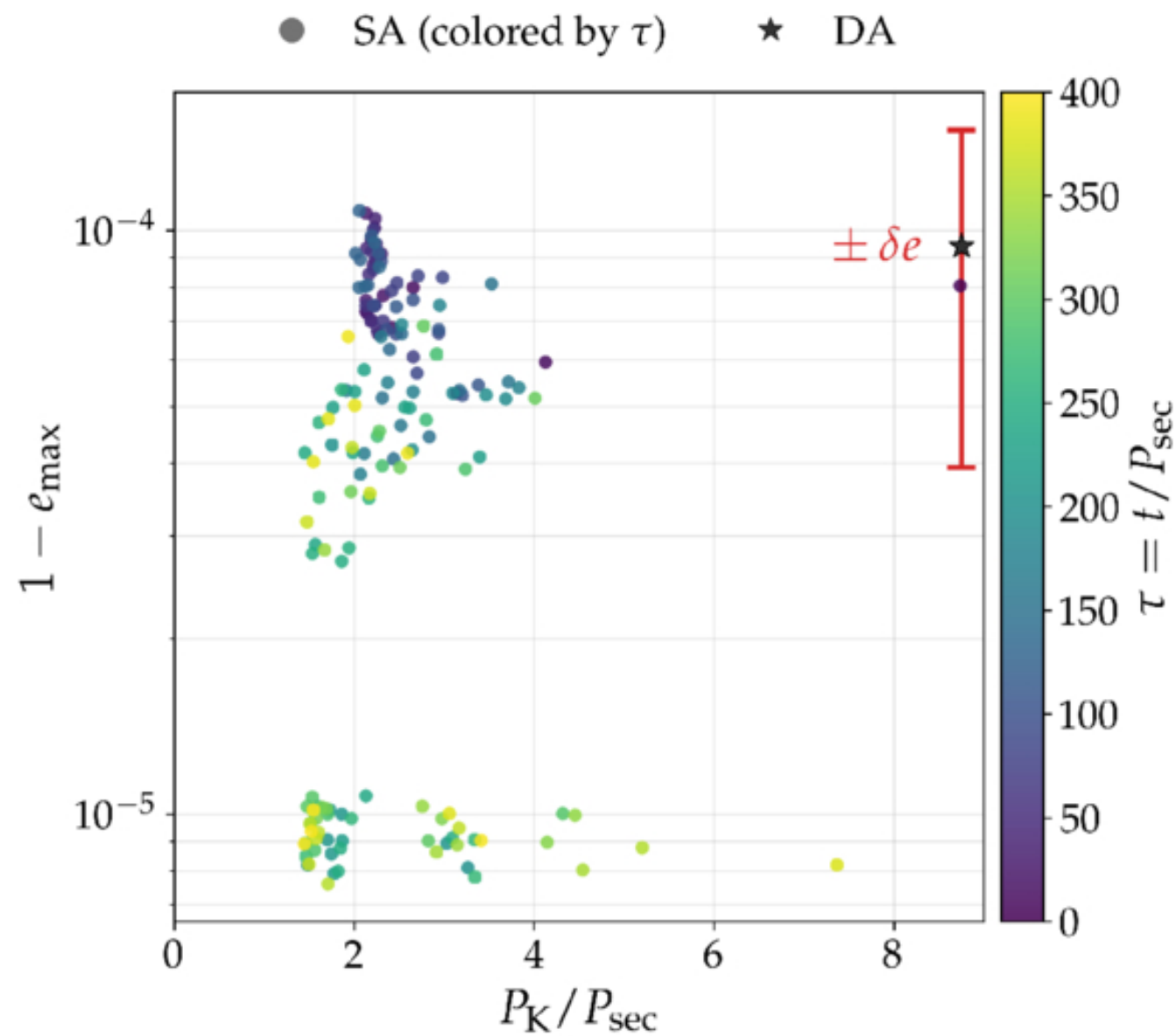
Figure 9. from Ygal Y. Klein and Chris Hamilton 2026 Astrophys. J. Lett. 1007 doi:10.3847/2041-8213/ae8ae8 https://dx.doi.org/10.3847/2041-8213/ae8ae8 © 2026. The Author(s). Published by the American Astronomical Society.
