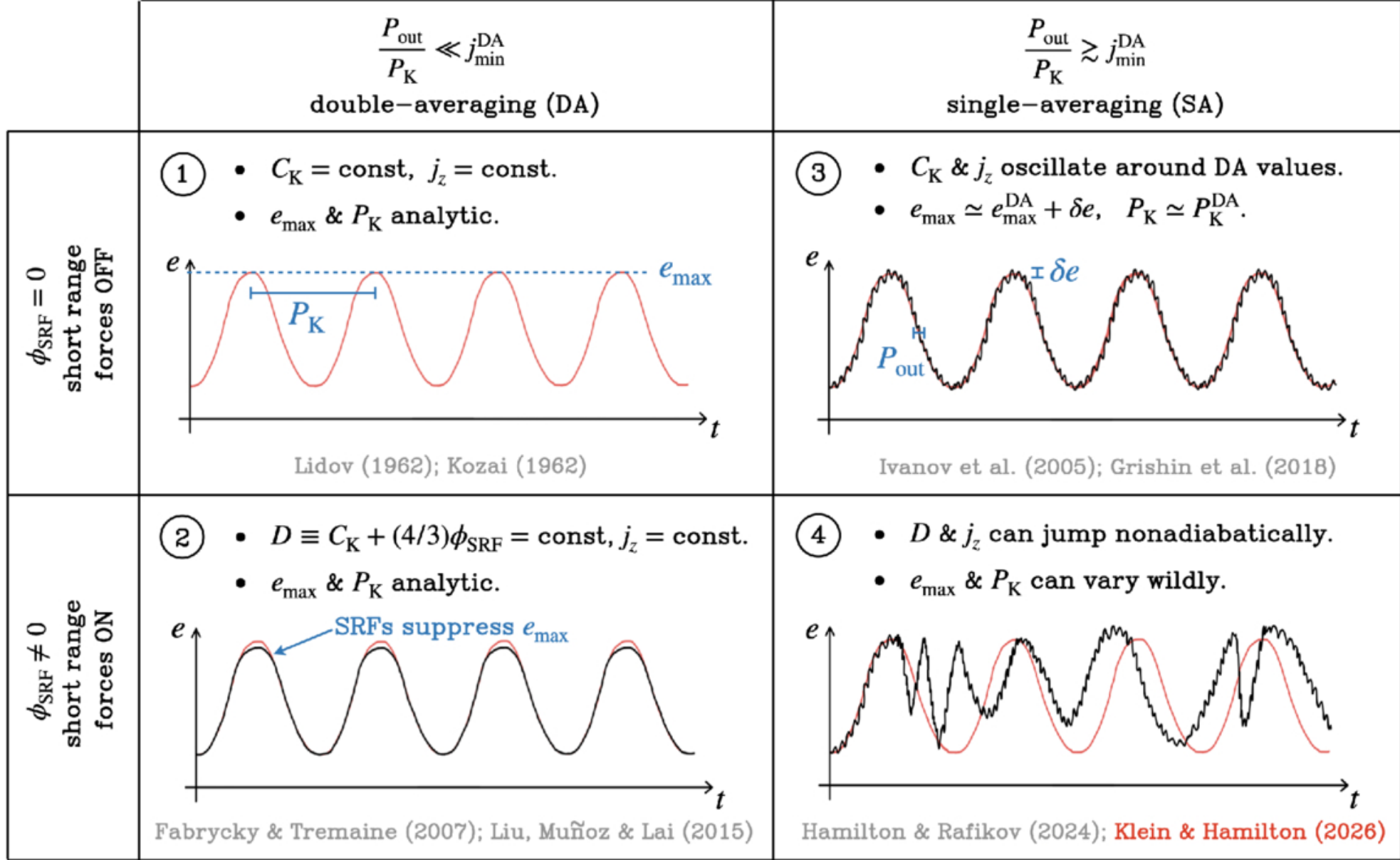
Figure 1. from Ygal Y. Klein and Chris Hamilton 2026 Astrophys. J. Lett. 1007 doi:10.3847/2041-8213/ae8ae8 https://dx.doi.org/10.3847/2041-8213/ae8ae8 © 2026. The Author(s). Published by the American Astronomical Society.
