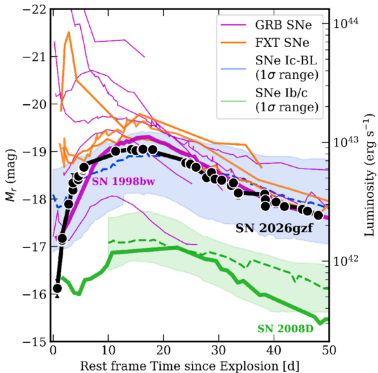
Figure 6. from Jillian C. Rastinejad et al 2026 Astrophys. J. Lett. 1007 doi:10.3847/2041-8213/ae8a4b https://dx.doi.org/10.3847/2041-8213/ae8a4b © 2026. The Author(s). Published by the American Astronomical Society.
