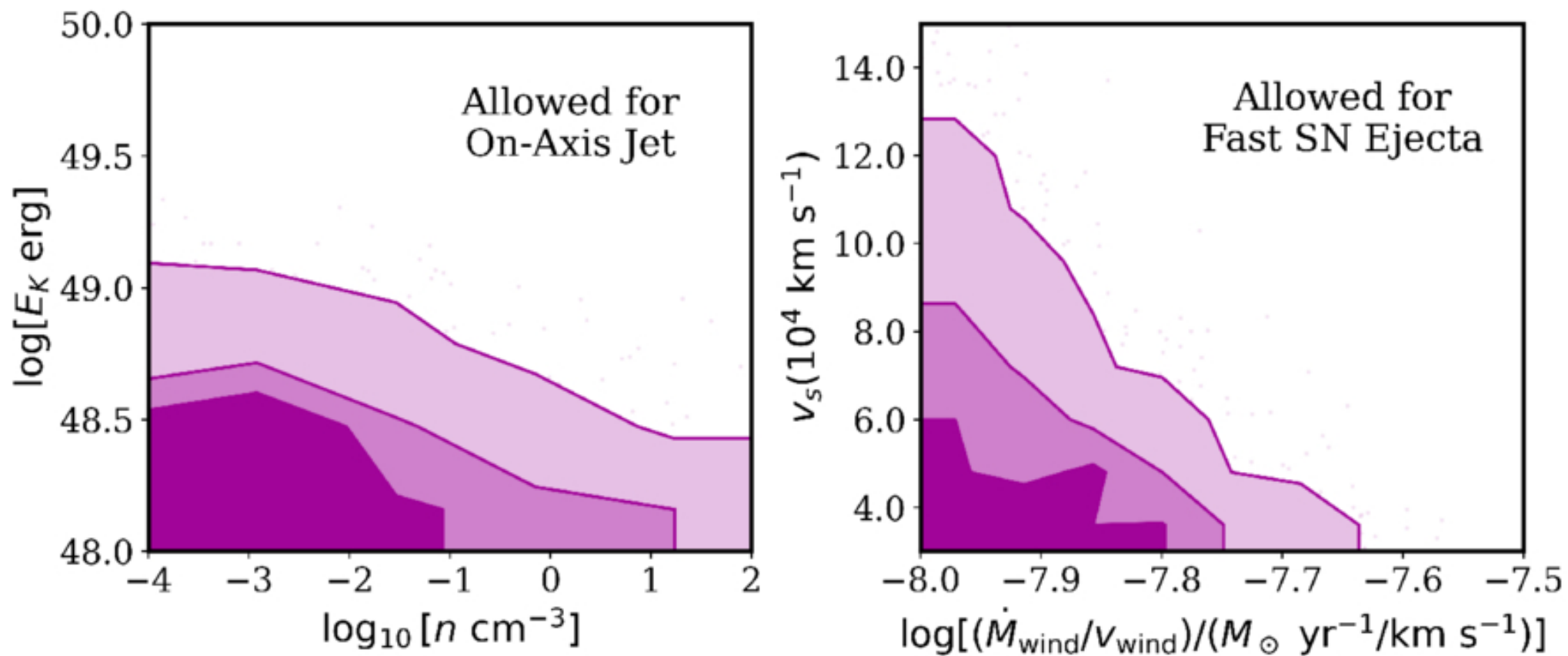
Figure 5. from Jillian C. Rastinejad et al 2026 Astrophys. J. Lett. 1007 doi:10.3847/2041-8213/ae8a4b https://dx.doi.org/10.3847/2041-8213/ae8a4b © 2026. The Author(s). Published by the American Astronomical Society.
