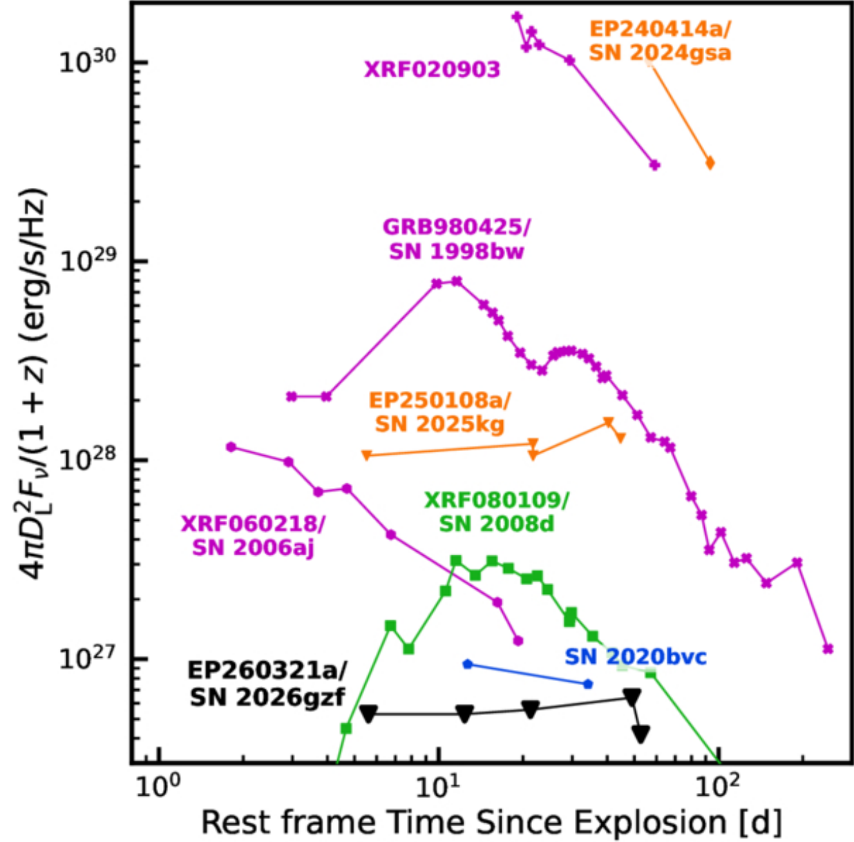
Figure 4. from Jillian C. Rastinejad et al 2026 Astrophys. J. Lett. 1007 doi:10.3847/2041-8213/ae8a4b https://dx.doi.org/10.3847/2041-8213/ae8a4b © 2026. The Author(s). Published by the American Astronomical Society.
