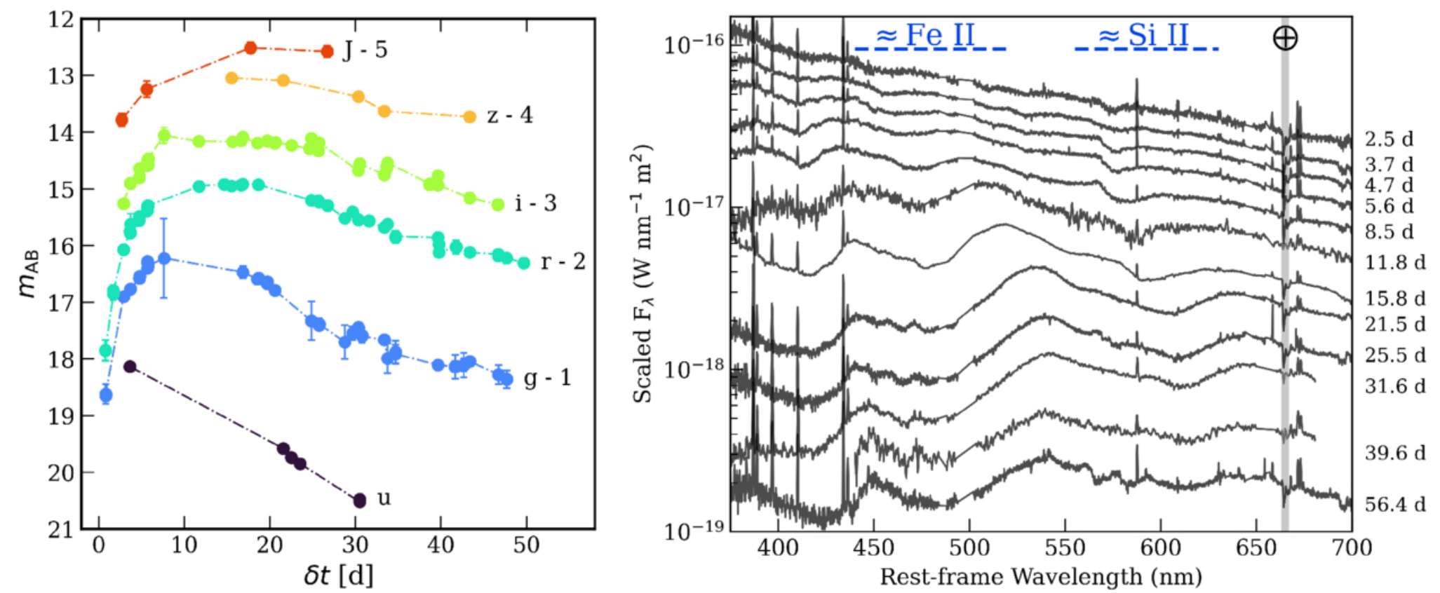
Figure 2. from Jillian C. Rastinejad et al 2026 Astrophys. J. Lett. 1007 doi:10.3847/2041-8213/ae8a4b https://dx.doi.org/10.3847/2041-8213/ae8a4b © 2026. The Author(s). Published by the American Astronomical Society.
