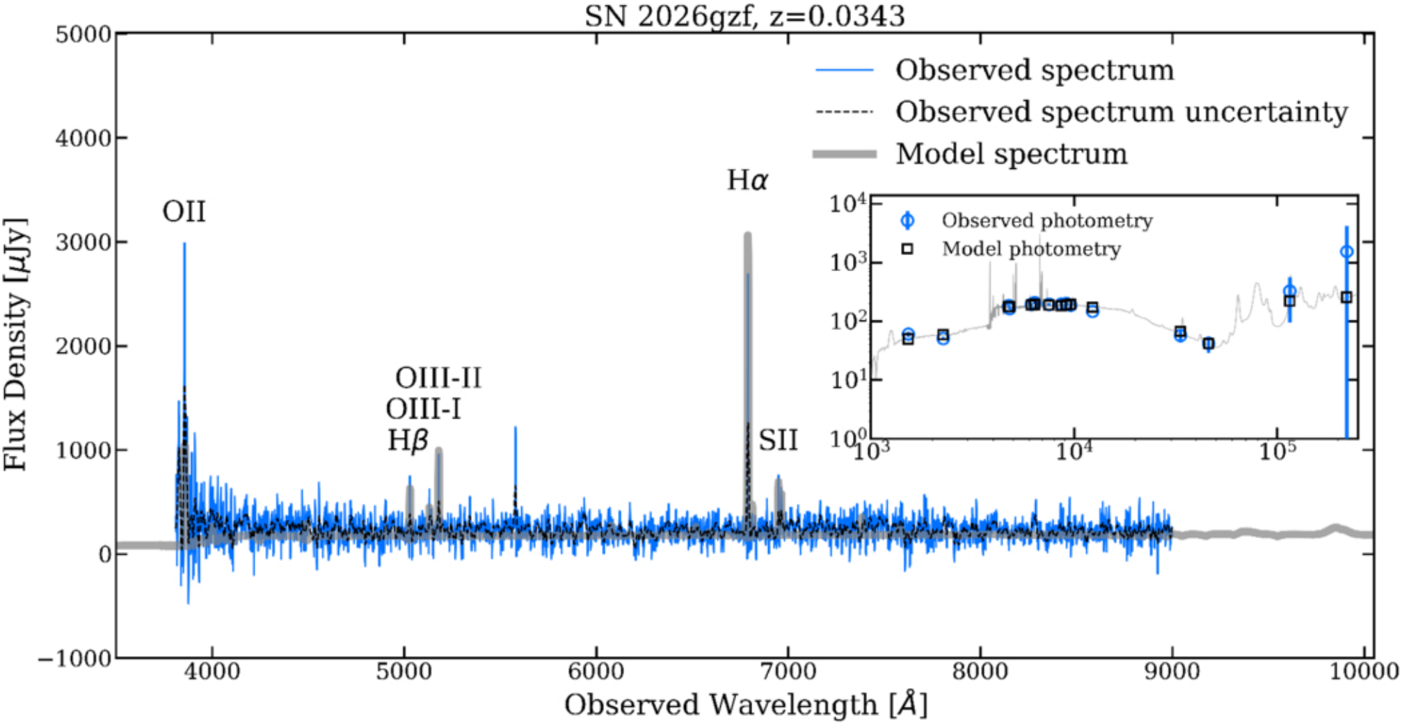
Figure 16. from Jillian C. Rastinejad et al 2026 Astrophys. J. Lett. 1007 doi:10.3847/2041-8213/ae8a4b https://dx.doi.org/10.3847/2041-8213/ae8a4b © 2026. The Author(s). Published by the American Astronomical Society.
