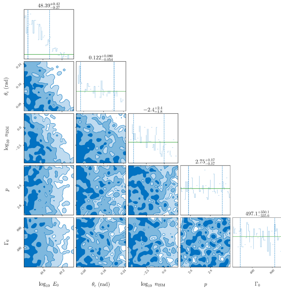
Figure 13. from Jillian C. Rastinejad et al 2026 Astrophys. J. Lett. 1007 doi:10.3847/2041-8213/ae8a4b https://dx.doi.org/10.3847/2041-8213/ae8a4b © 2026. The Author(s). Published by the American Astronomical Society.
