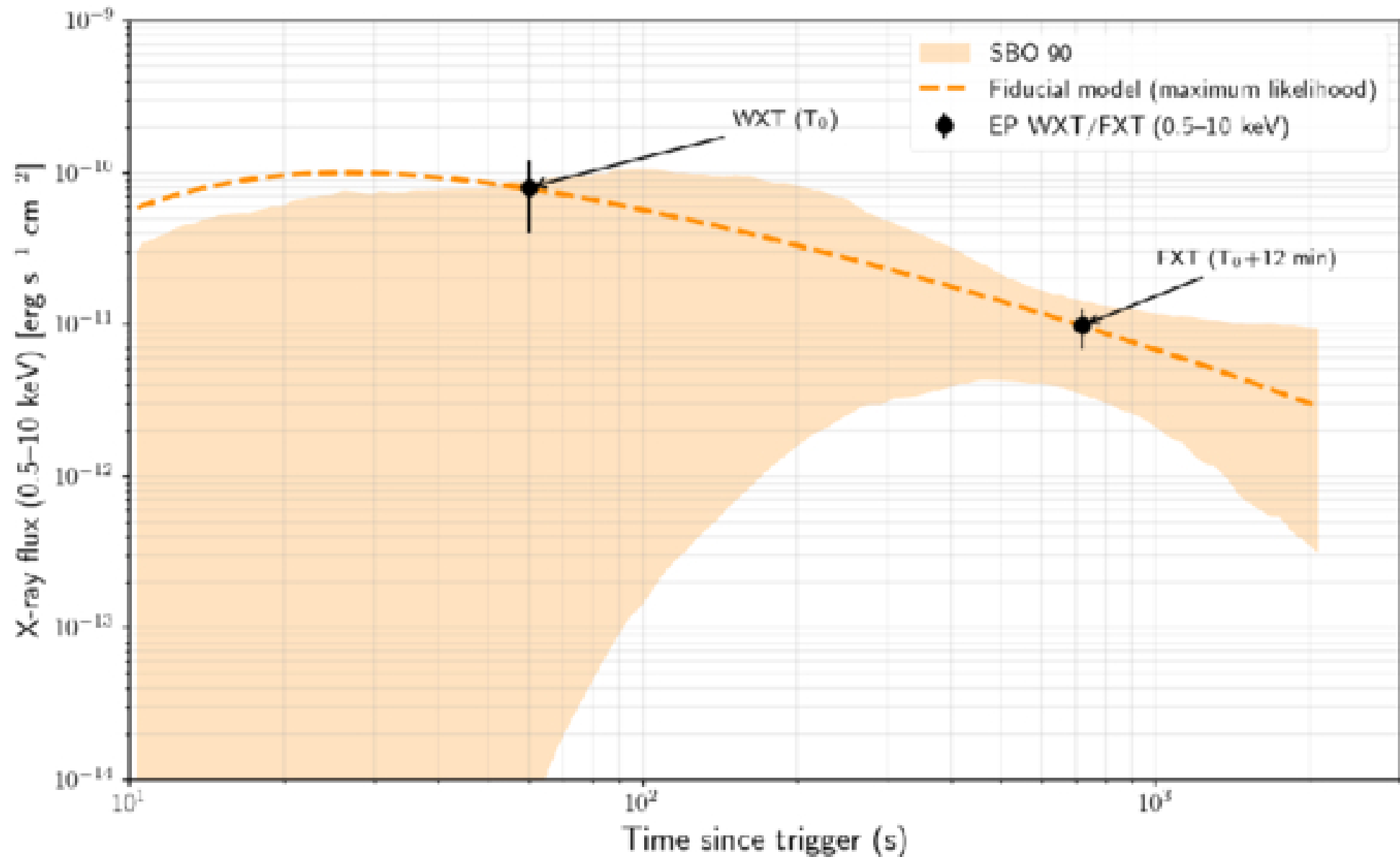
Figure 12. from Jillian C. Rastinejad et al 2026 Astrophys. J. Lett. 1007 doi:10.3847/2041-8213/ae8a4b https://dx.doi.org/10.3847/2041-8213/ae8a4b © 2026. The Author(s). Published by the American Astronomical Society.
