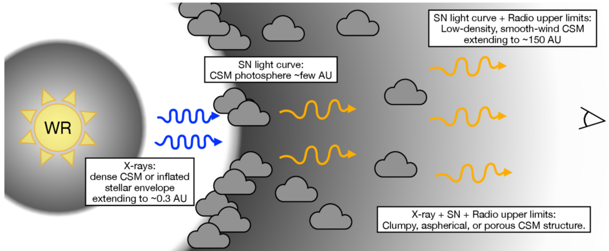
Figure 11. from Jillian C. Rastinejad et al 2026 Astrophys. J. Lett. 1007 doi:10.3847/2041-8213/ae8a4b https://dx.doi.org/10.3847/2041-8213/ae8a4b © 2026. The Author(s). Published by the American Astronomical Society.
