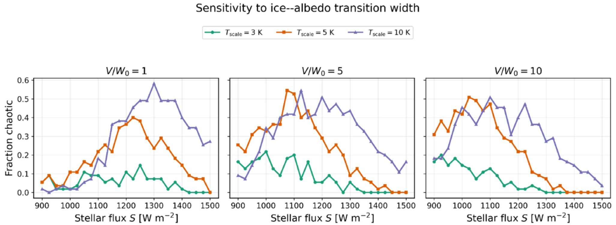
Figure 8. from Chaucer Langbert et al 2026 Astrophys. J. Lett. 1006 doi:10.3847/2041-8213/ae8a43 https://dx.doi.org/10.3847/2041-8213/ae8a43 © 2026. The Author(s). Published by the American Astronomical Society.
