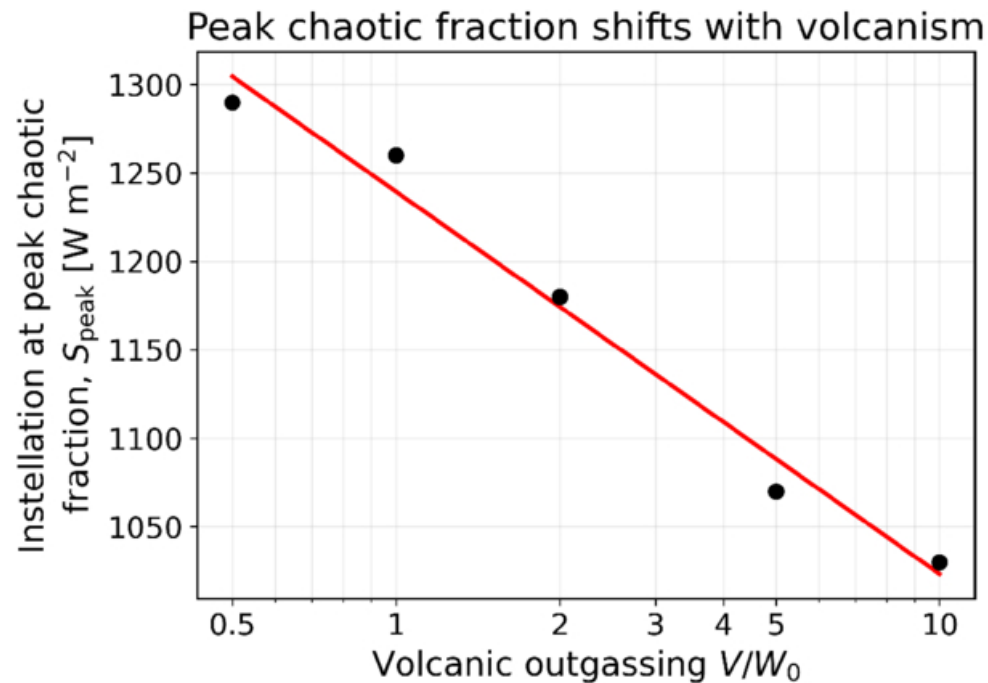
Figure 5. from Chaucer Langbert et al 2026 Astrophys. J. Lett. 1006 doi:10.3847/2041-8213/ae8a43 https://dx.doi.org/10.3847/2041-8213/ae8a43 © 2026. The Author(s). Published by the American Astronomical Society.
