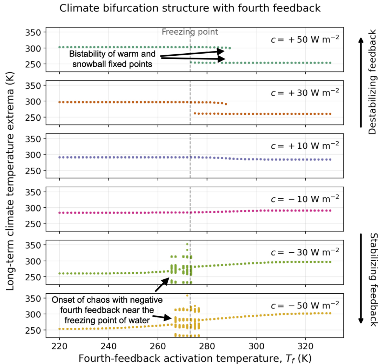
Figure 3. from Chaucer Langbert et al 2026 Astrophys. J. Lett. 1006 doi:10.3847/2041-8213/ae8a43 https://dx.doi.org/10.3847/2041-8213/ae8a43 © 2026. The Author(s). Published by the American Astronomical Society.
