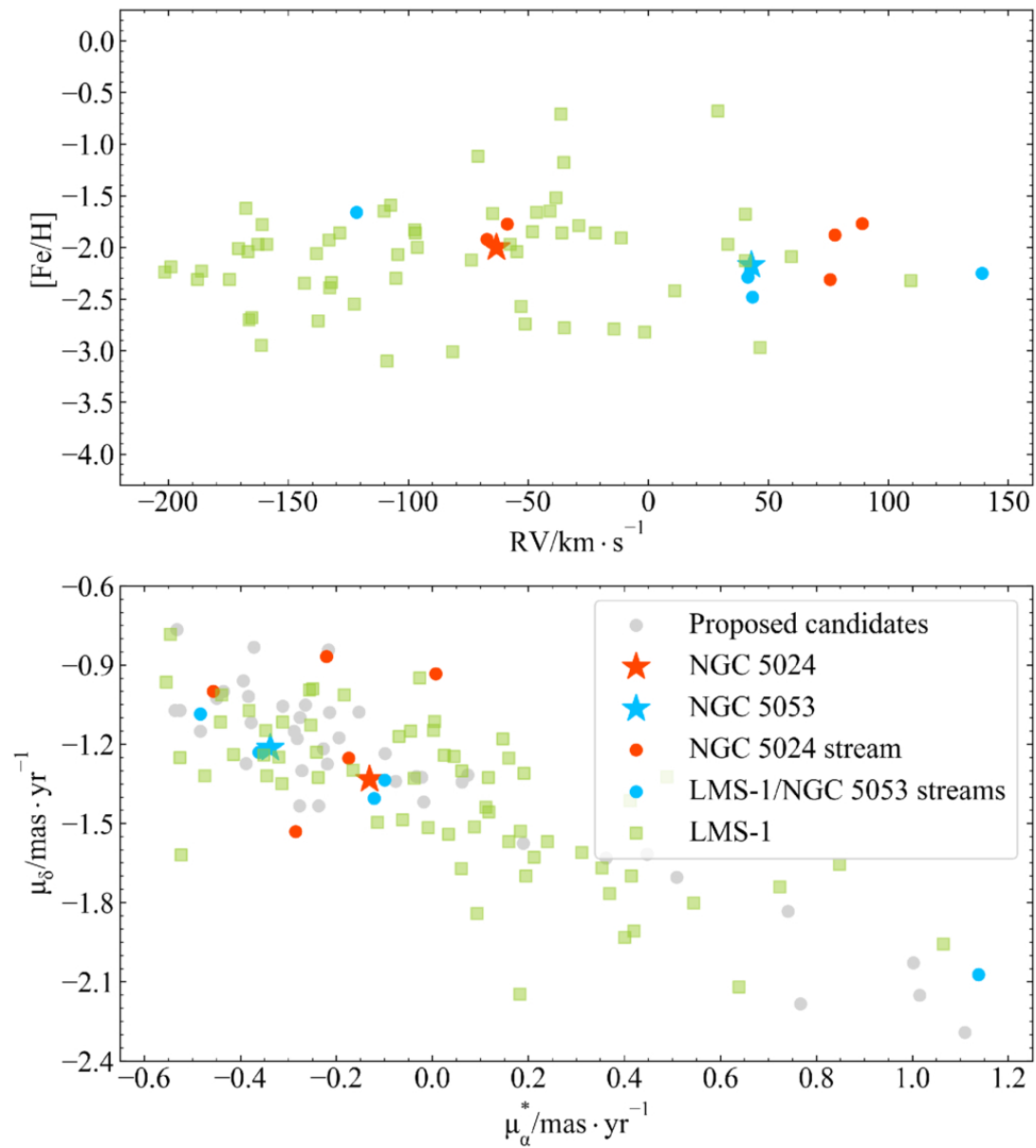
Figure 5. from Xianhao Ye et al 2026 Astrophys. J. Lett. 1006 doi:10.3847/2041-8213/ae89b8 https://dx.doi.org/10.3847/2041-8213/ae89b8 © 2026. The Author(s). Published by the American Astronomical Society.
