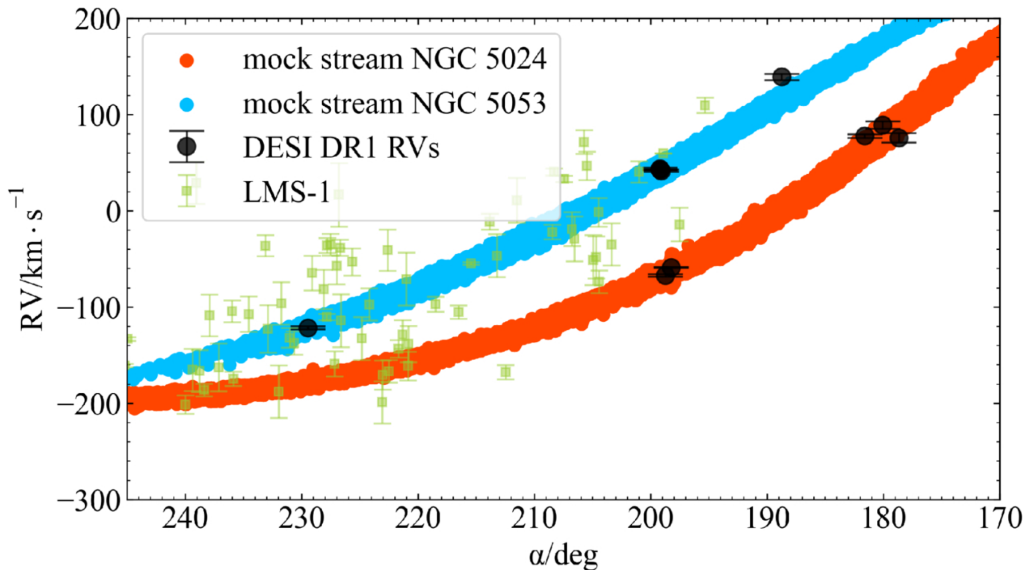
Figure 4. from Xianhao Ye et al 2026 Astrophys. J. Lett. 1006 doi:10.3847/2041-8213/ae89b8 https://dx.doi.org/10.3847/2041-8213/ae89b8 © 2026. The Author(s). Published by the American Astronomical Society.
