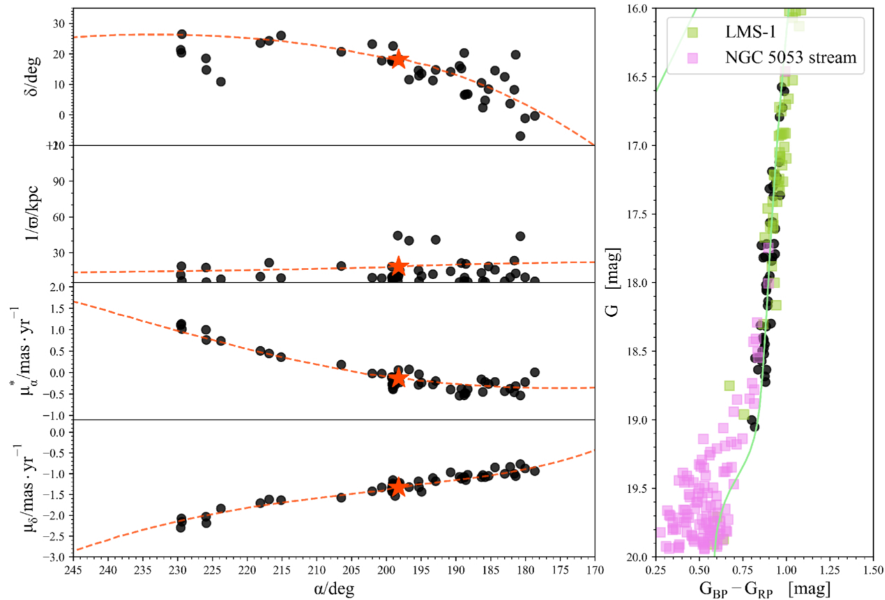
Figure 3. from Xianhao Ye et al 2026 Astrophys. J. Lett. 1006 doi:10.3847/2041-8213/ae89b8 https://dx.doi.org/10.3847/2041-8213/ae89b8 © 2026. The Author(s). Published by the American Astronomical Society.
