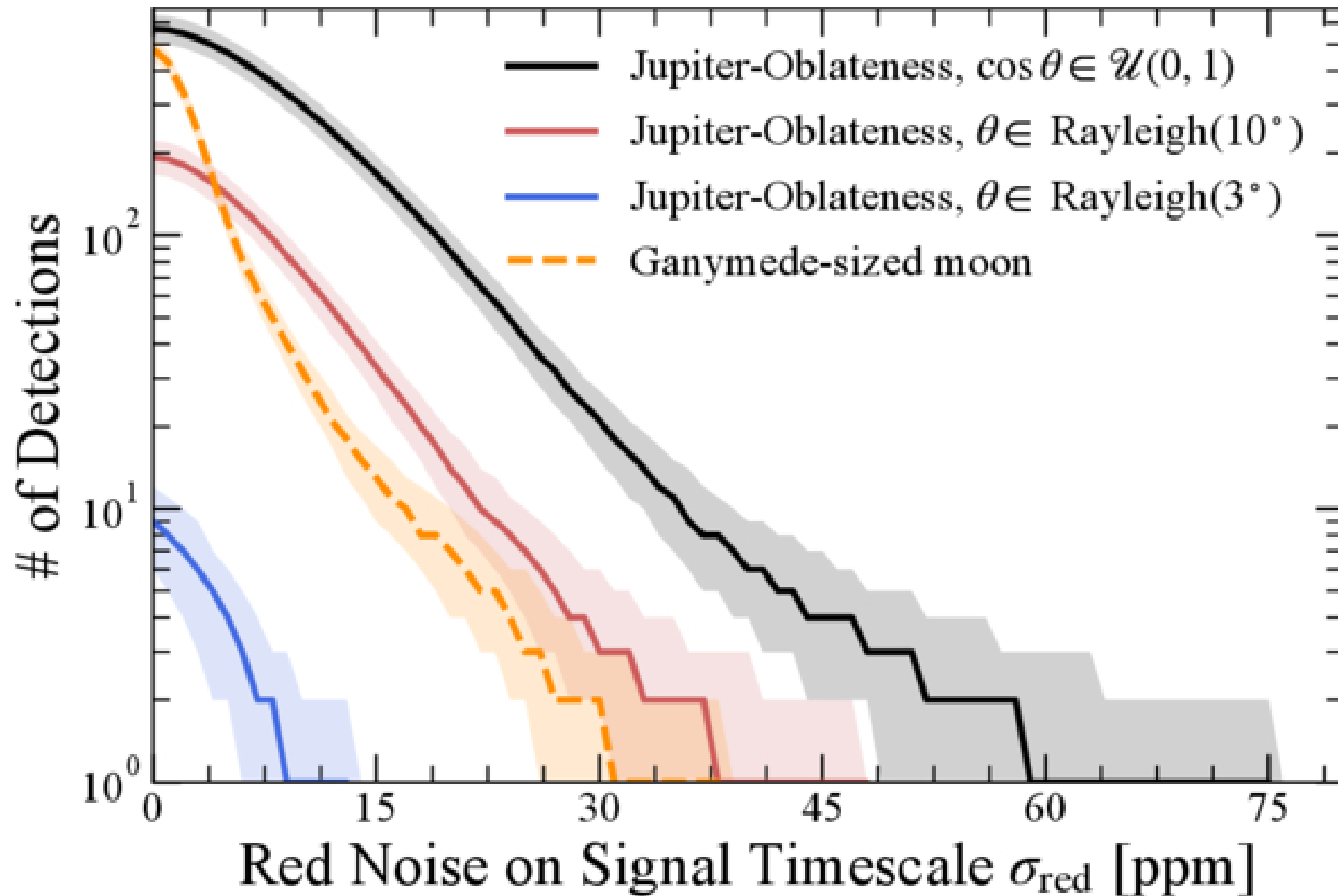
Figure 8. from Le-Chris Wang et al 2026 Astrophys. J. Lett. 1006 doi:10.3847/2041-8213/ae89a6 https://dx.doi.org/10.3847/2041-8213/ae89a6 © 2026. The Author(s). Published by the American Astronomical Society.
