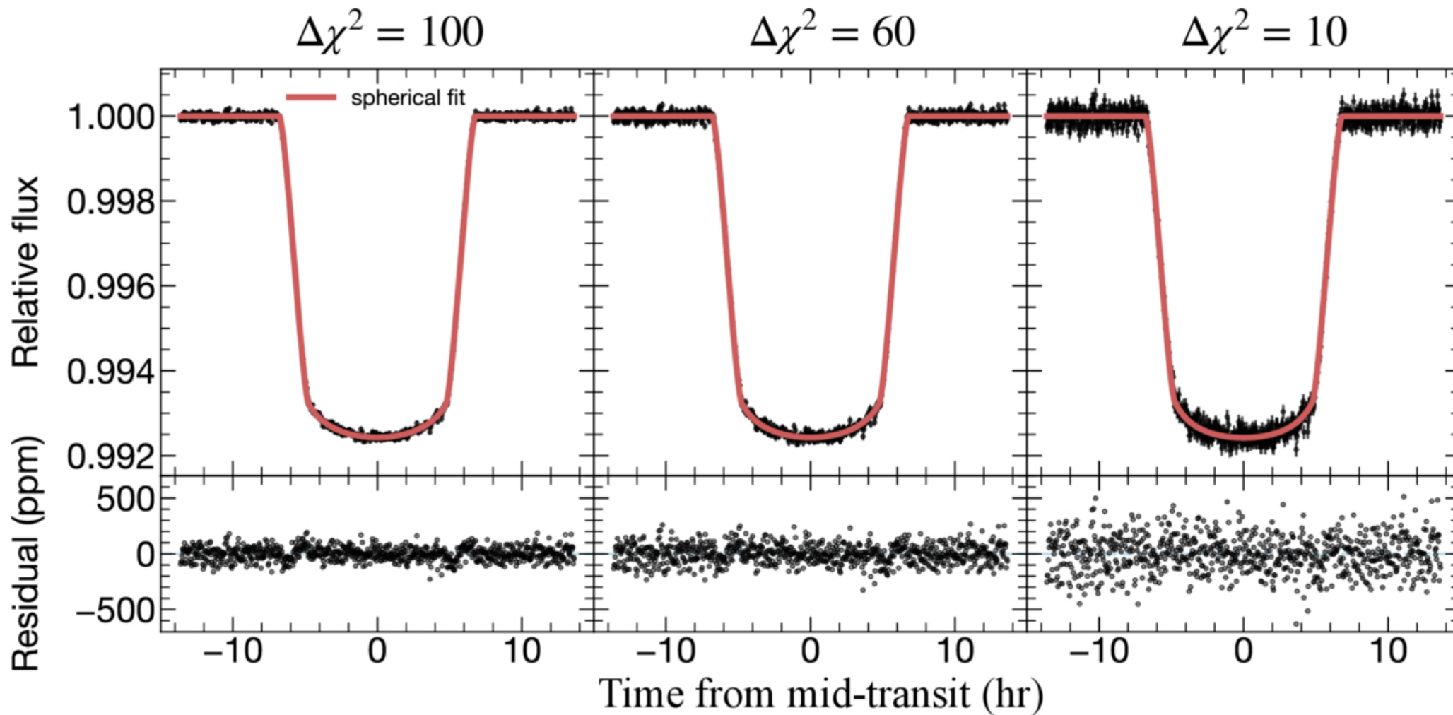
Figure 4. from Le-Chris Wang et al 2026 Astrophys. J. Lett. 1006 doi:10.3847/2041-8213/ae89a6 https://dx.doi.org/10.3847/2041-8213/ae89a6 © 2026. The Author(s). Published by the American Astronomical Society.
