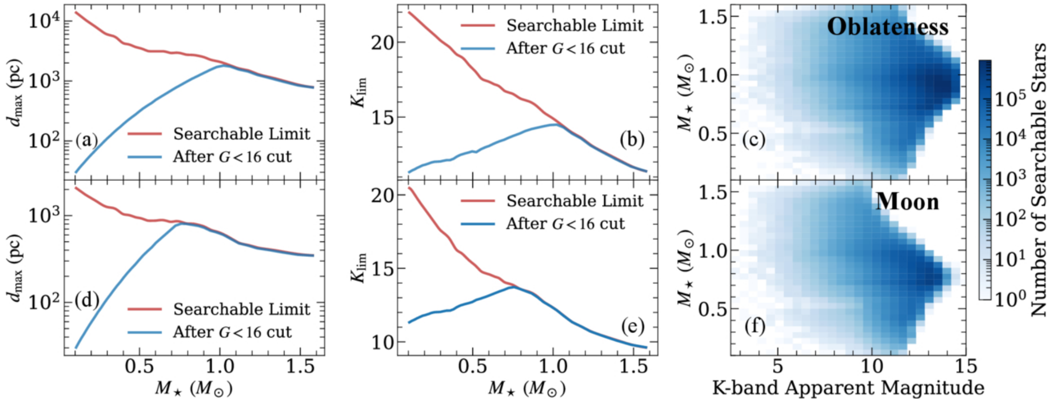
Figure 3. from Le-Chris Wang et al 2026 Astrophys. J. Lett. 1006 doi:10.3847/2041-8213/ae89a6 https://dx.doi.org/10.3847/2041-8213/ae89a6 © 2026. The Author(s). Published by the American Astronomical Society.
