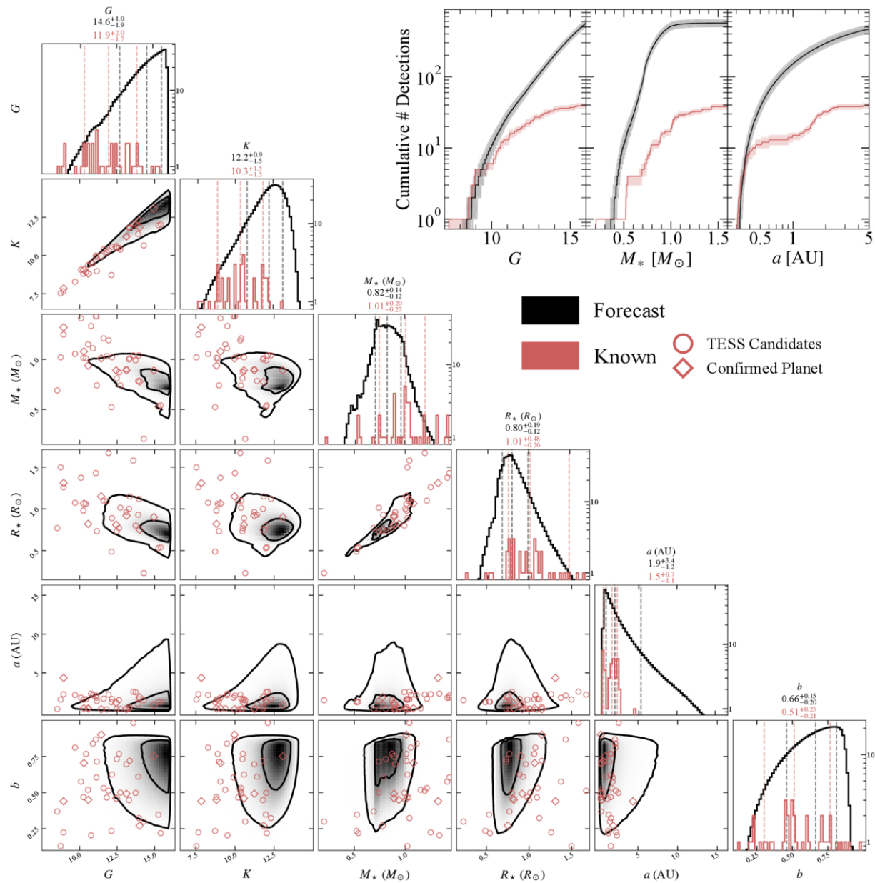
Figure 10. from Le-Chris Wang et al 2026 Astrophys. J. Lett. 1006 doi:10.3847/2041-8213/ae89a6 https://dx.doi.org/10.3847/2041-8213/ae89a6 © 2026. The Author(s). Published by the American Astronomical Society.
