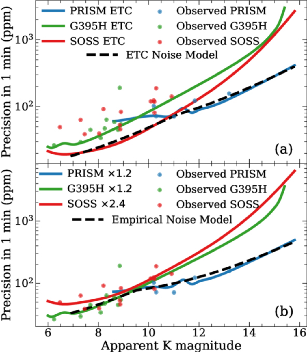
Figure 1. from Le-Chris Wang et al 2026 Astrophys. J. Lett. 1006 doi:10.3847/2041-8213/ae89a6 https://dx.doi.org/10.3847/2041-8213/ae89a6 © 2026. The Author(s). Published by the American Astronomical Society.
