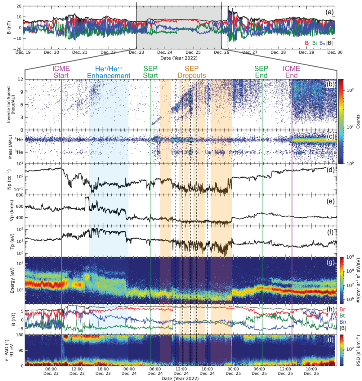
Figure 5. from Radoslav Buík et al 2026 Astrophys. J. Lett. 1006 doi:10.3847/2041-8213/ae8994 https://dx.doi.org/10.3847/2041-8213/ae8994 © 2026. The Author(s). Published by the American Astronomical Society.
