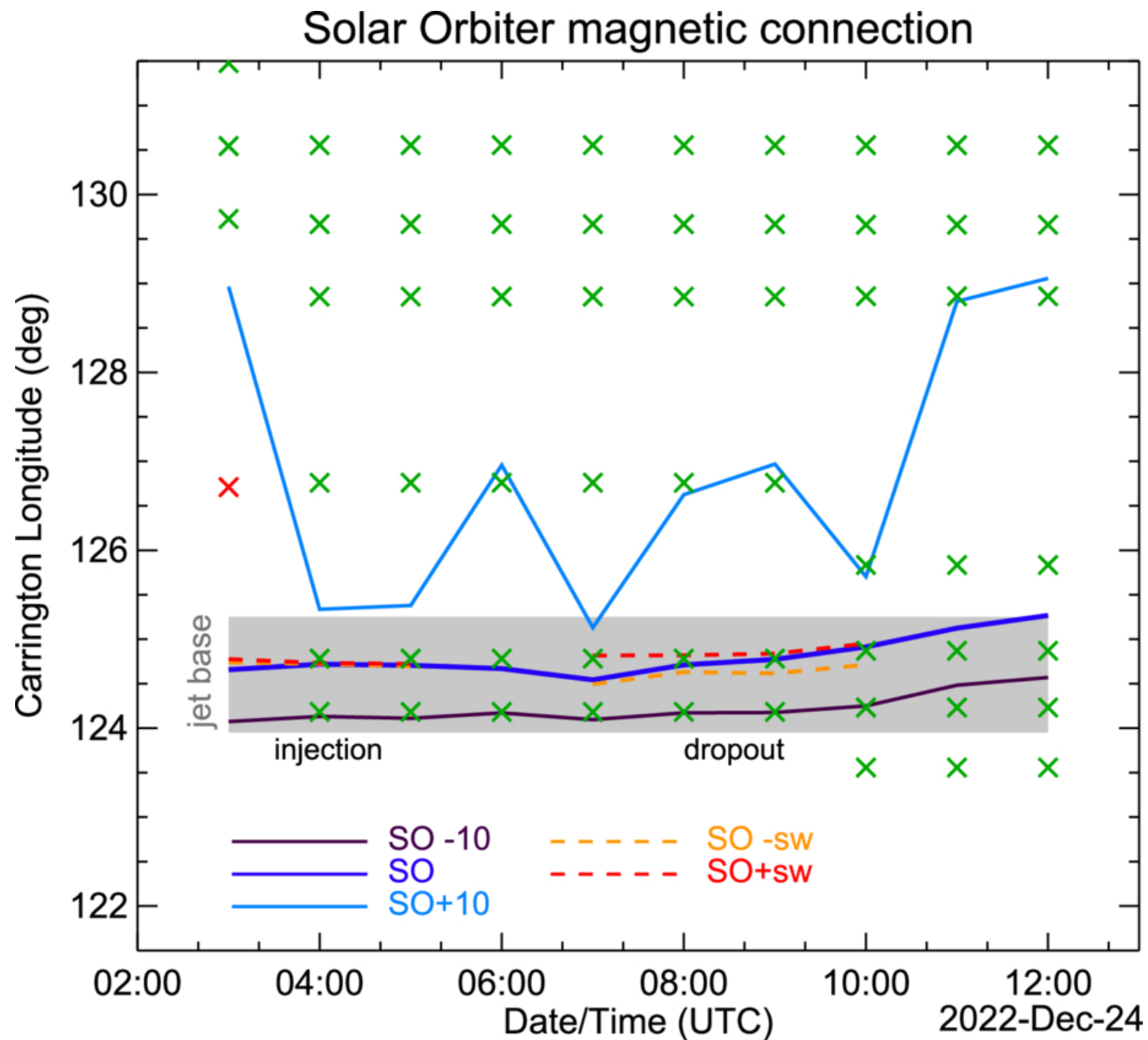
Figure 4. from Radoslav Buík et al 2026 Astrophys. J. Lett. 1006 doi:10.3847/2041-8213/ae8994 https://dx.doi.org/10.3847/2041-8213/ae8994 © 2026. The Author(s). Published by the American Astronomical Society.
