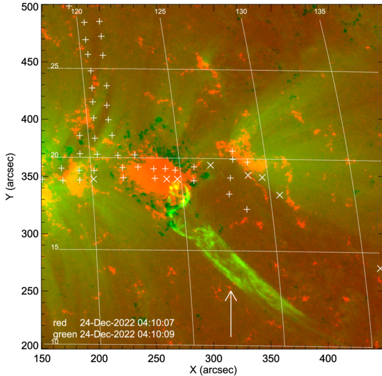
Figure 2. from Radoslav Buík et al 2026 Astrophys. J. Lett. 1006 doi:10.3847/2041-8213/ae8994 https://dx.doi.org/10.3847/2041-8213/ae8994 © 2026. The Author(s). Published by the American Astronomical Society.
