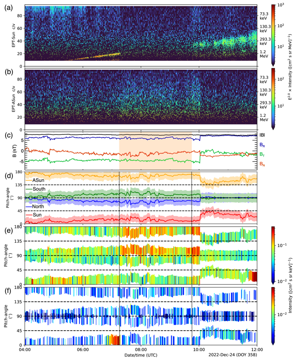
Figure 1. from Radoslav Buík et al 2026 Astrophys. J. Lett. 1006 doi:10.3847/2041-8213/ae8994 https://dx.doi.org/10.3847/2041-8213/ae8994 © 2026. The Author(s). Published by the American Astronomical Society.
