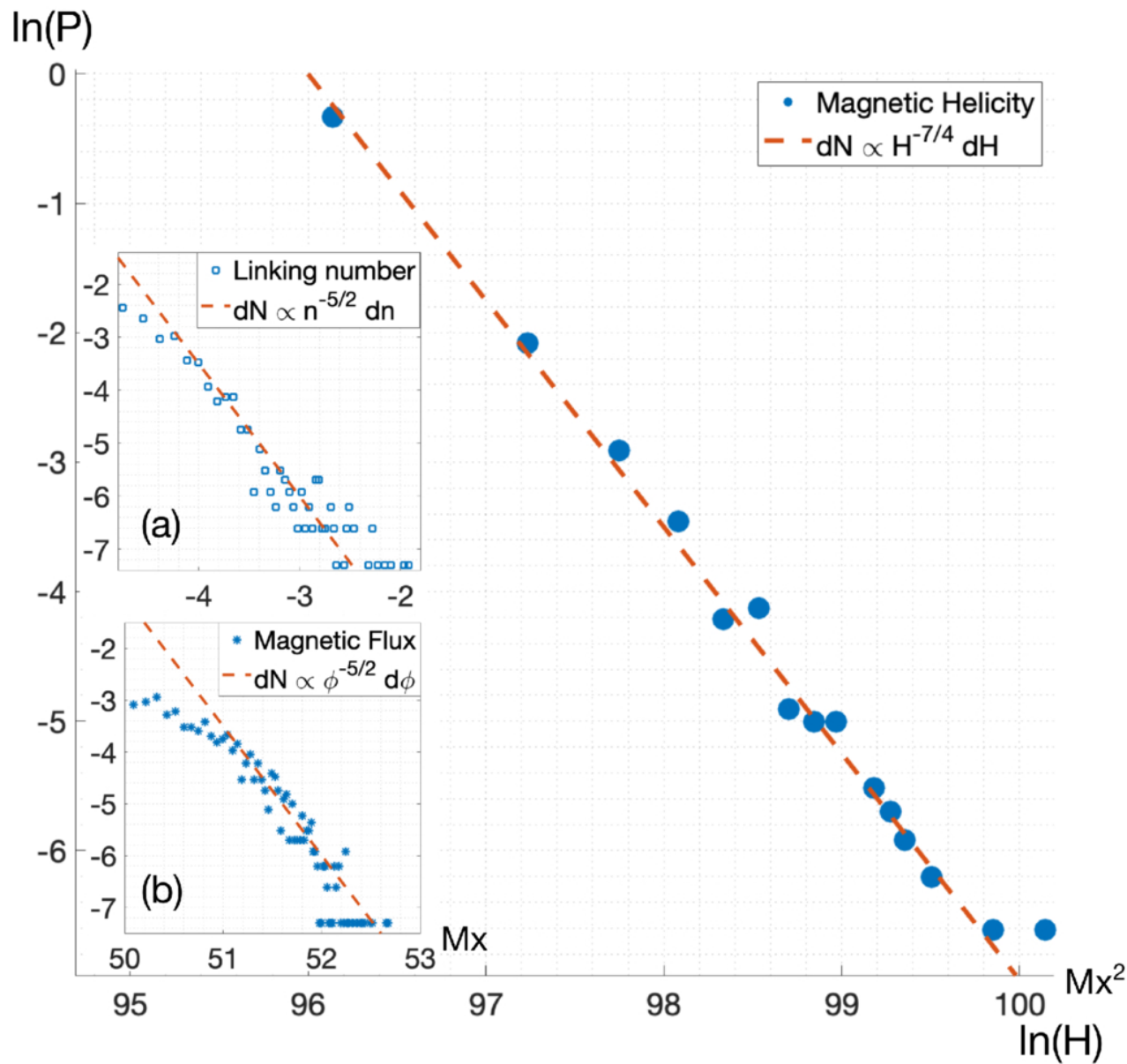
Figure 3. from Anda Xiong et al 2026 Astrophys. J. Lett. 1006 doi:10.3847/2041-8213/ae8992 https://dx.doi.org/10.3847/2041-8213/ae8992 © 2026. The Author(s). Published by the American Astronomical Society.
