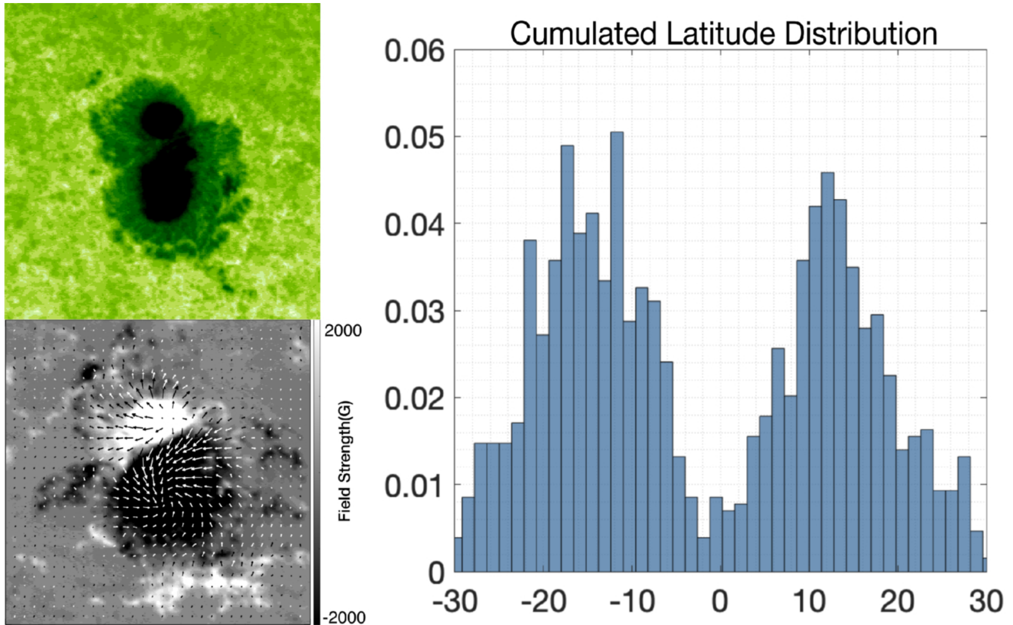
Figure 1. from Anda Xiong et al 2026 Astrophys. J. Lett. 1006 doi:10.3847/2041-8213/ae8992 https://dx.doi.org/10.3847/2041-8213/ae8992 © 2026. The Author(s). Published by the American Astronomical Society.
