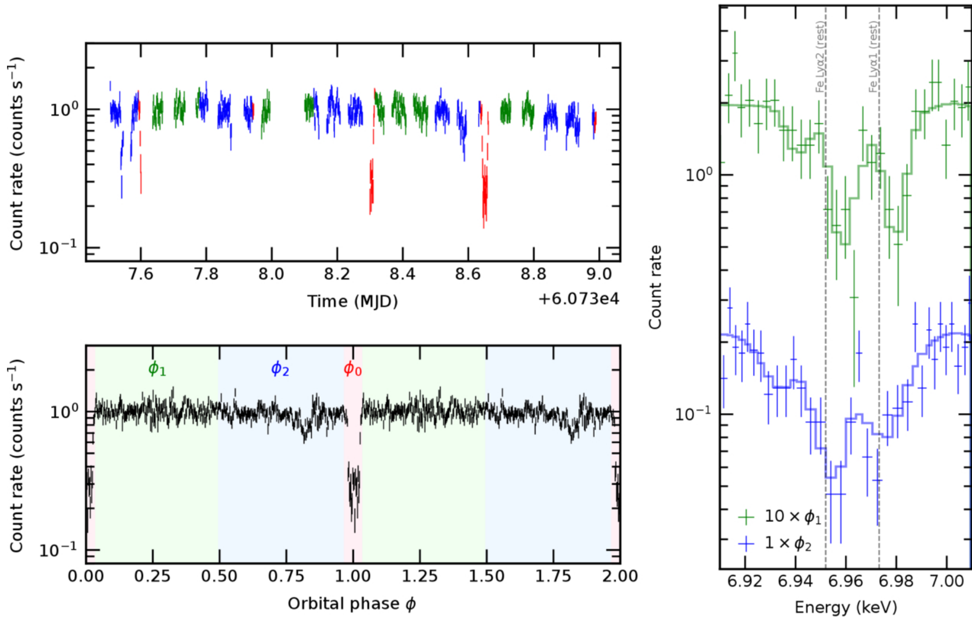
Figure 4. from Kai Matsunaga et al 2026 Astrophys. J. Lett. 1006 doi:10.3847/2041-8213/ae8907 https://dx.doi.org/10.3847/2041-8213/ae8907 © 2026. The Author(s). Published by the American Astronomical Society.
