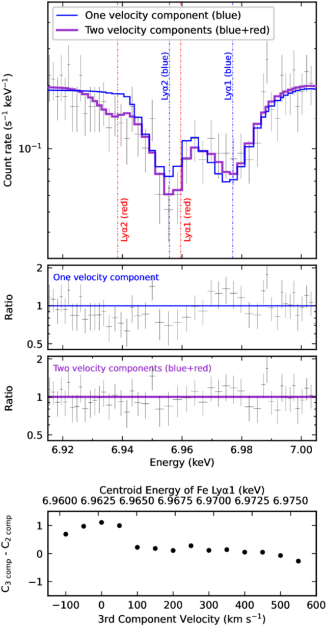
Figure 3. from Kai Matsunaga et al 2026 Astrophys. J. Lett. 1006 doi:10.3847/2041-8213/ae8907 https://dx.doi.org/10.3847/2041-8213/ae8907 © 2026. The Author(s). Published by the American Astronomical Society.
