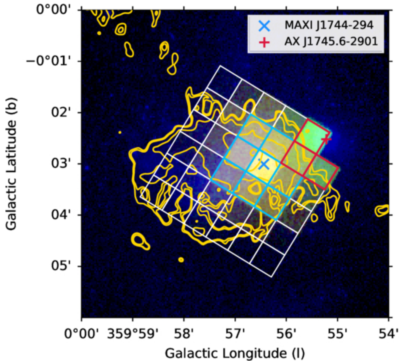
Figure 1. from Kai Matsunaga et al 2026 Astrophys. J. Lett. 1006 doi:10.3847/2041-8213/ae8907 https://dx.doi.org/10.3847/2041-8213/ae8907 © 2026. The Author(s). Published by the American Astronomical Society.
