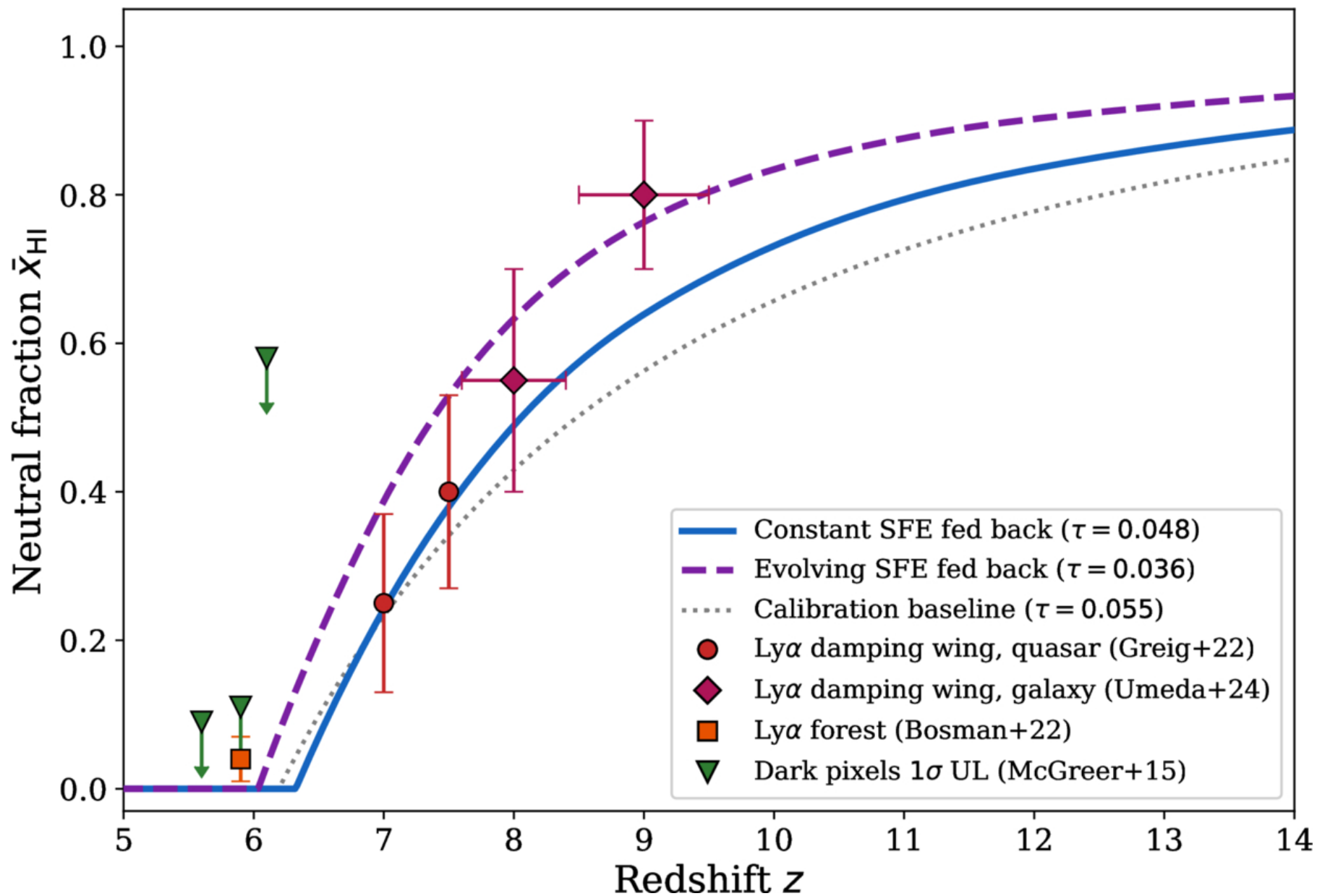
Figure 5. from Zihan Wang and Huanyuan Shan 2026 Astrophys. J. Lett. 1006 doi:10.3847/2041-8213/ae88f1 https://dx.doi.org/10.3847/2041-8213/ae88f1 © 2026. The Author(s). Published by the American Astronomical Society.
